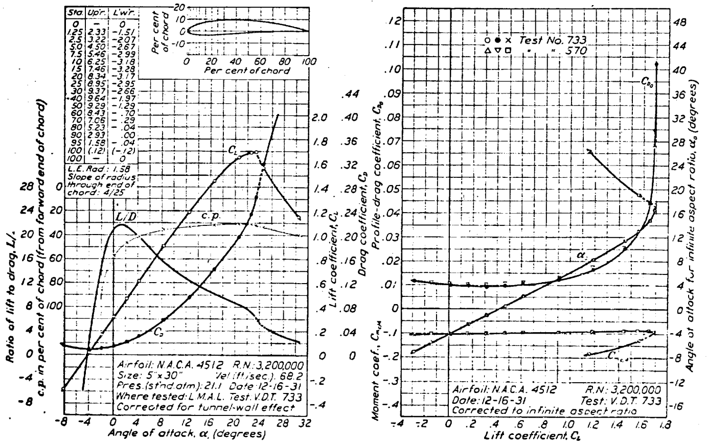
FIGURE 45.—N.A.C.A. 4512 airfoil.
