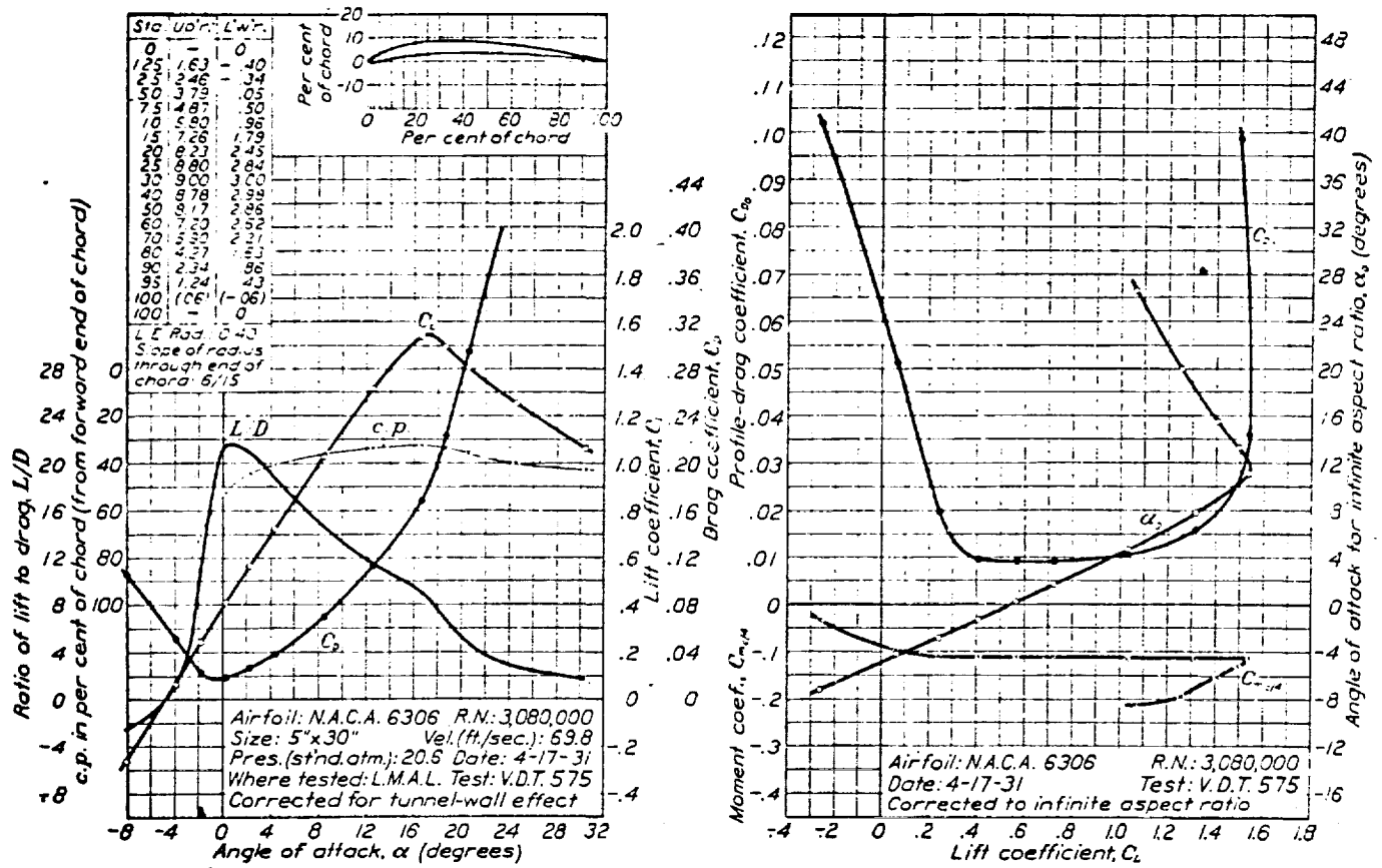
FIGURE 52.—N.A.C.A. 6306 airfoil.
