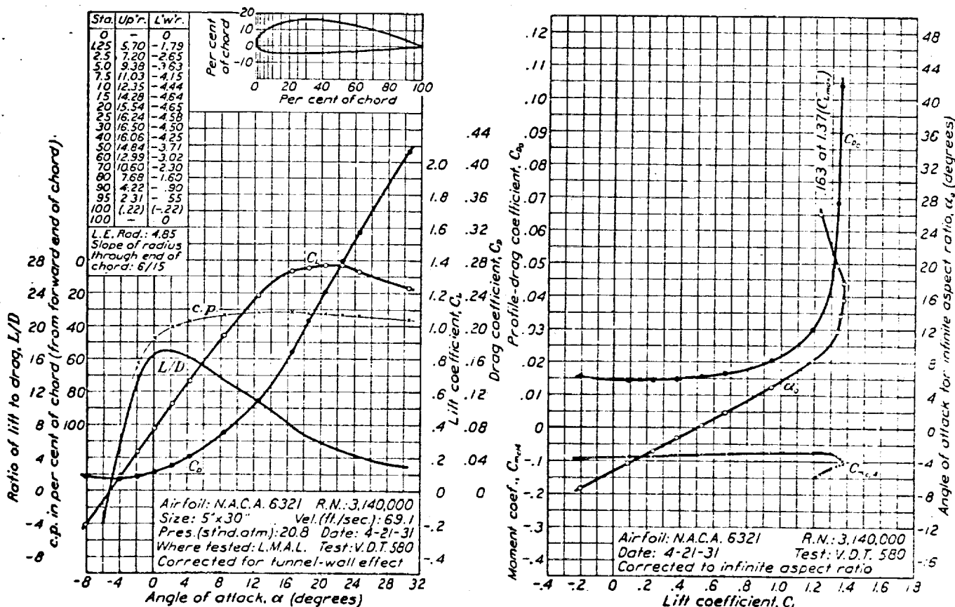
FIGURE 57.—N.A.C.A. 6321 airfoil.
