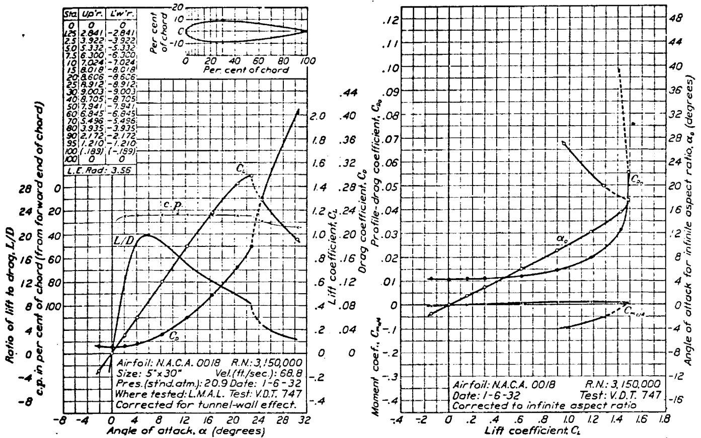
FIGURE 8.—N.A.C.A. 0018 airfoil.
