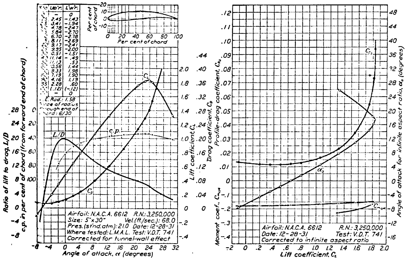
FIGURE 70.—N.A.C.A. 6612 airfoil.
