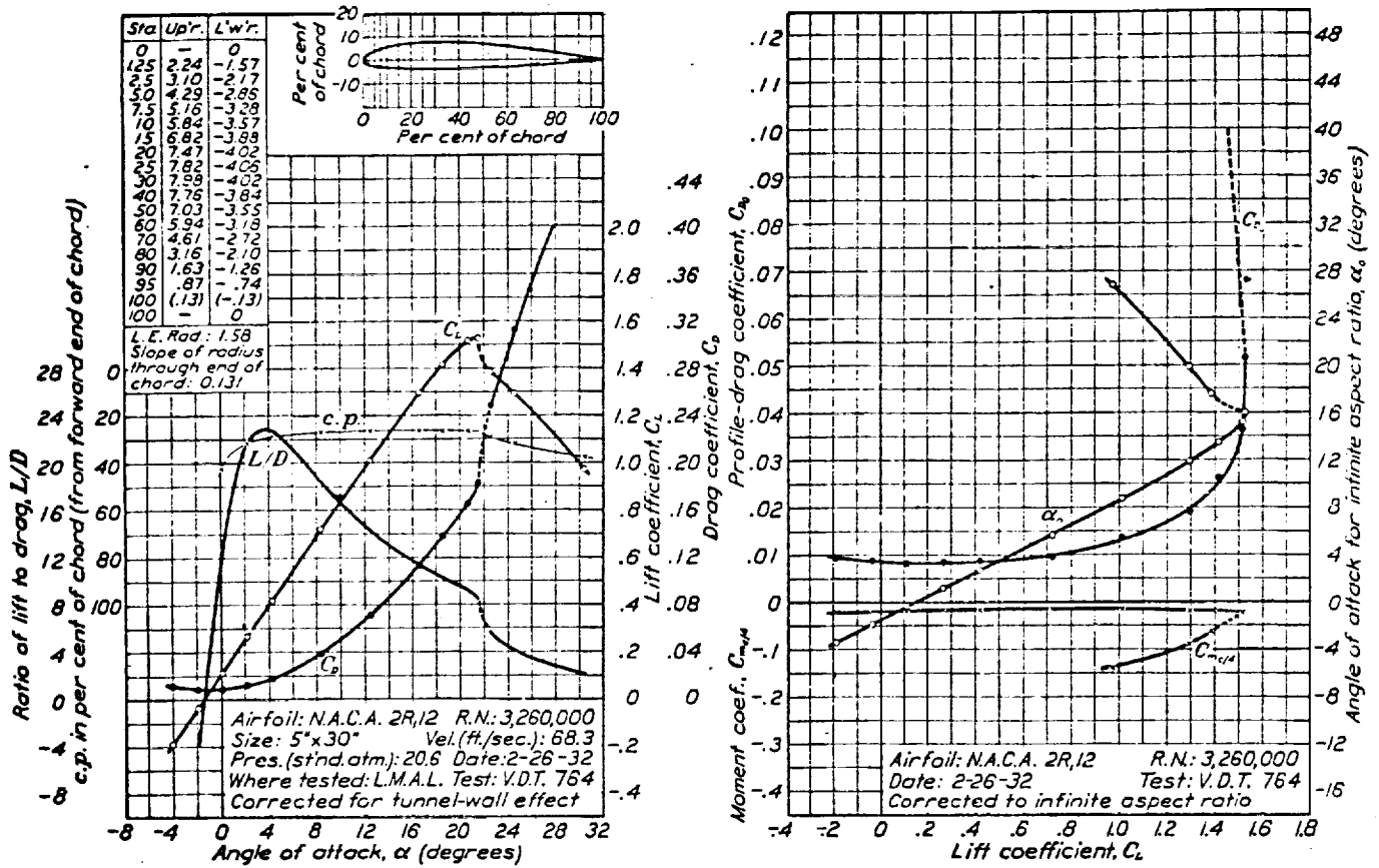
FIGURE 78.—N.A.C.A. 2R 12 airfoil.
