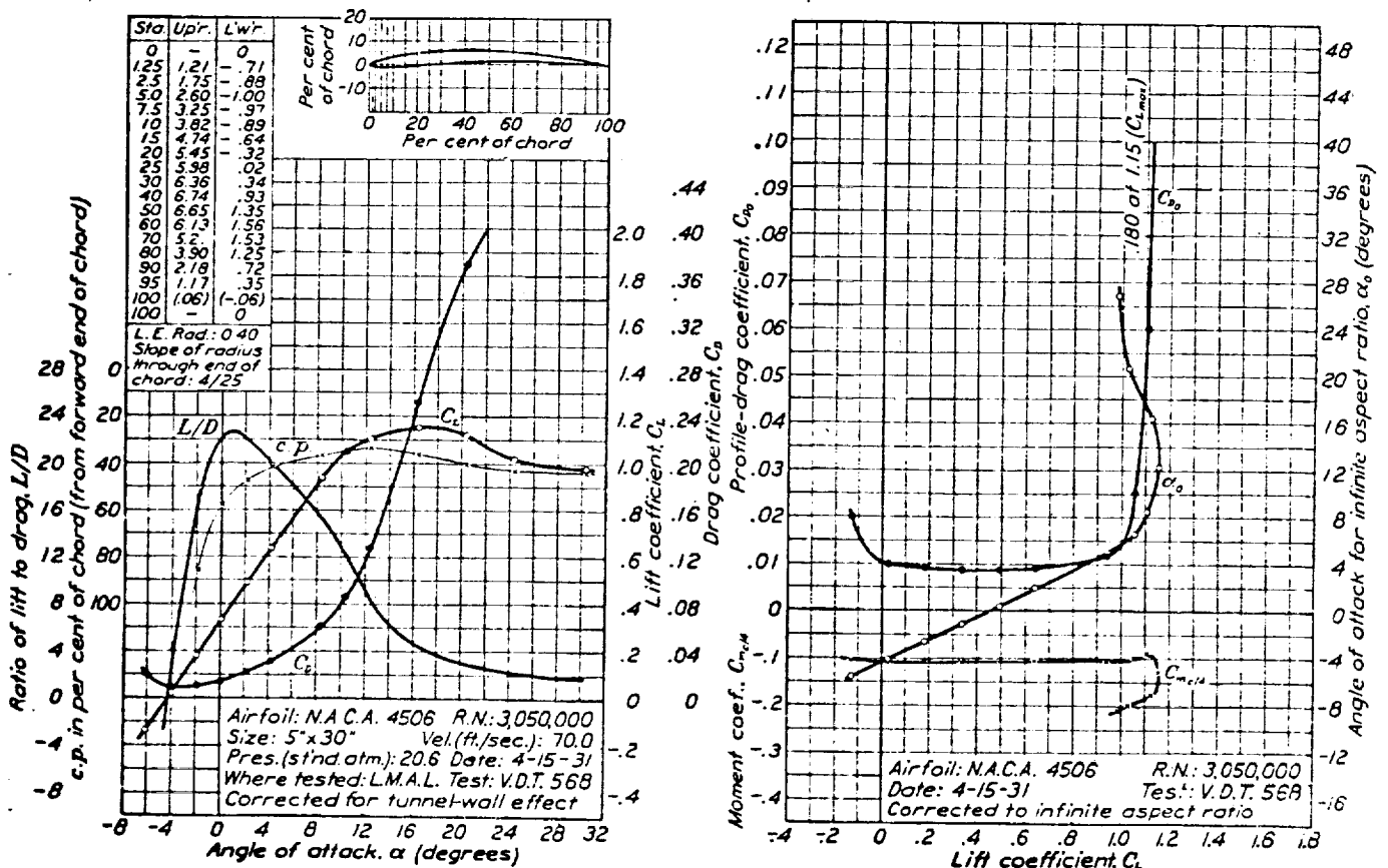
FIGURE 43.—N.A.C.A. 4506 airfoil.
