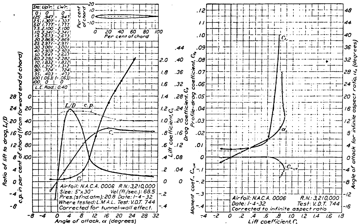
FIGURE 4.—N.A.C.A. 0006 airfoil.
