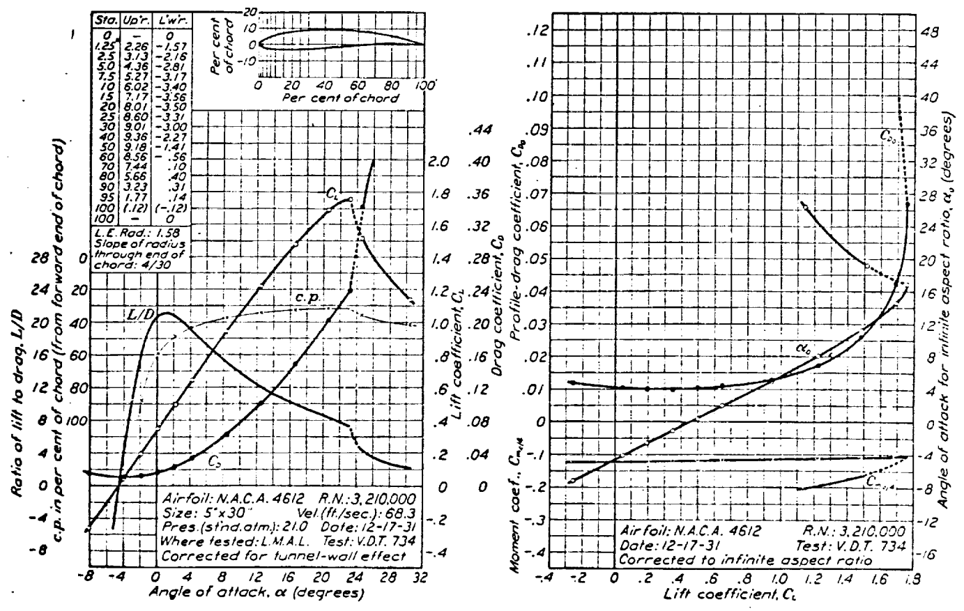
FIGURE 49.—N.A.C.A. 4612 airfoil.
