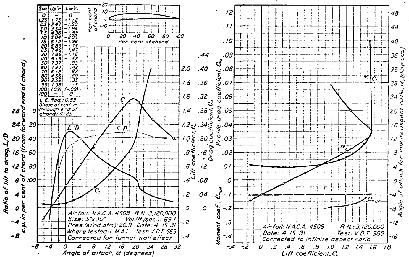
FIGURE 44.—N.A.C.A. 4509 airfoil.
