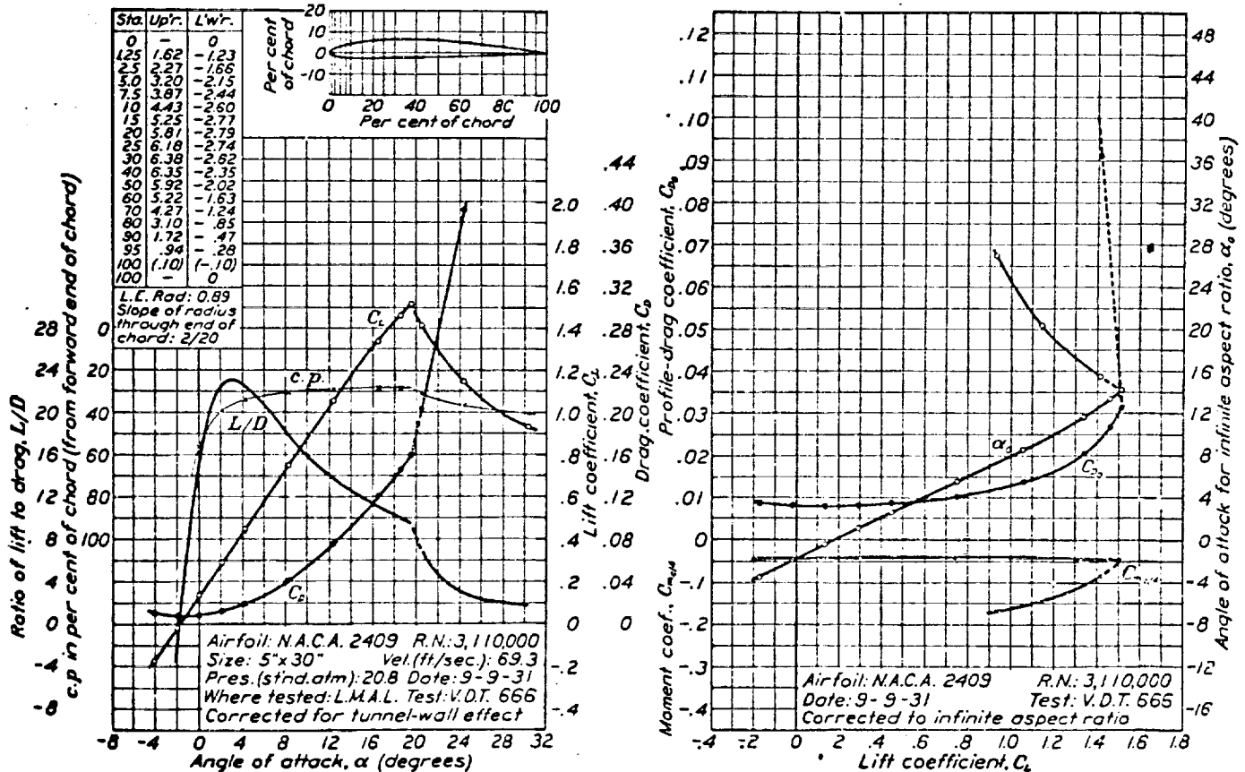
FIGURE 17.—N.A.C.A. 2409 airfoil.
