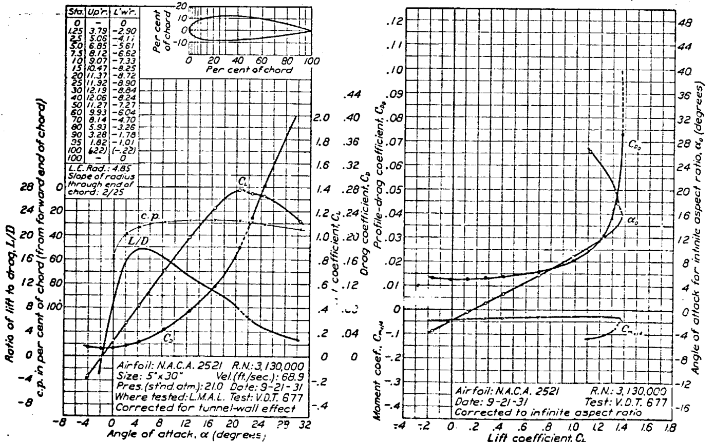
FIGURE 27.—N.A.C.A. 2521 airfoil.
