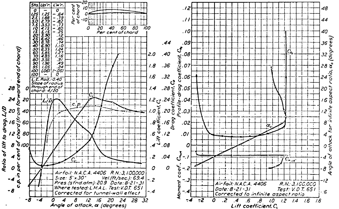
FIGURE 37.—N.A.C.A. 4406 airfoil.
