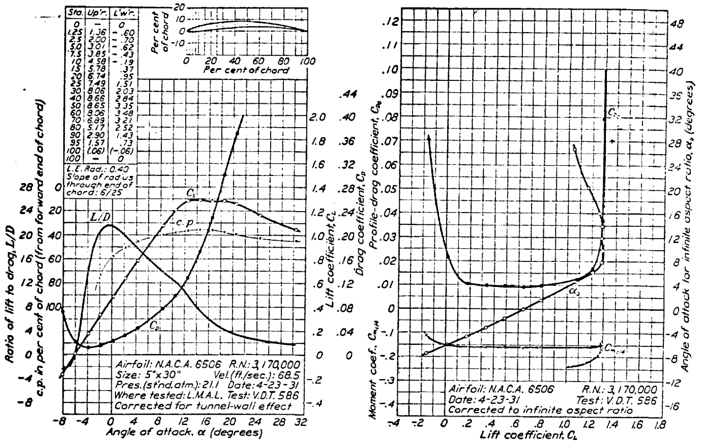
FIGURE 64.—N.A.C.A. 6506 airfoil.
