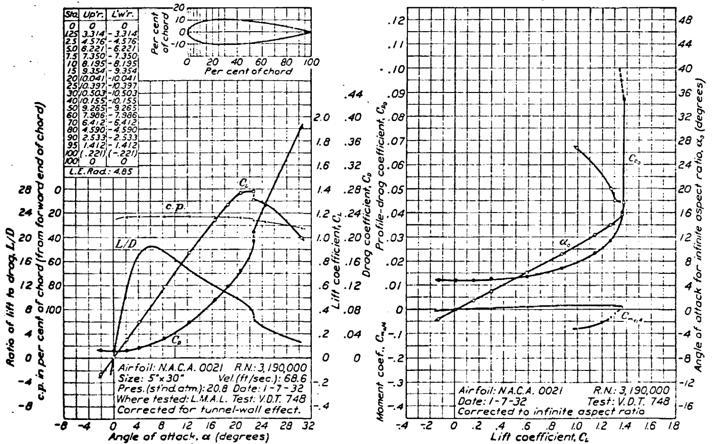
FIGURE 9.—N.A.C.A. 0021 airfoil.
