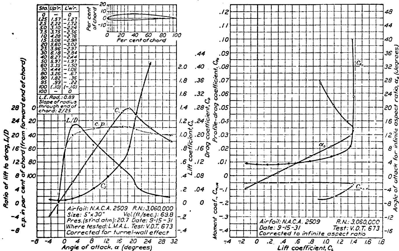
FIGURE 23.—N.A.C.A. 2509 airfoil.
