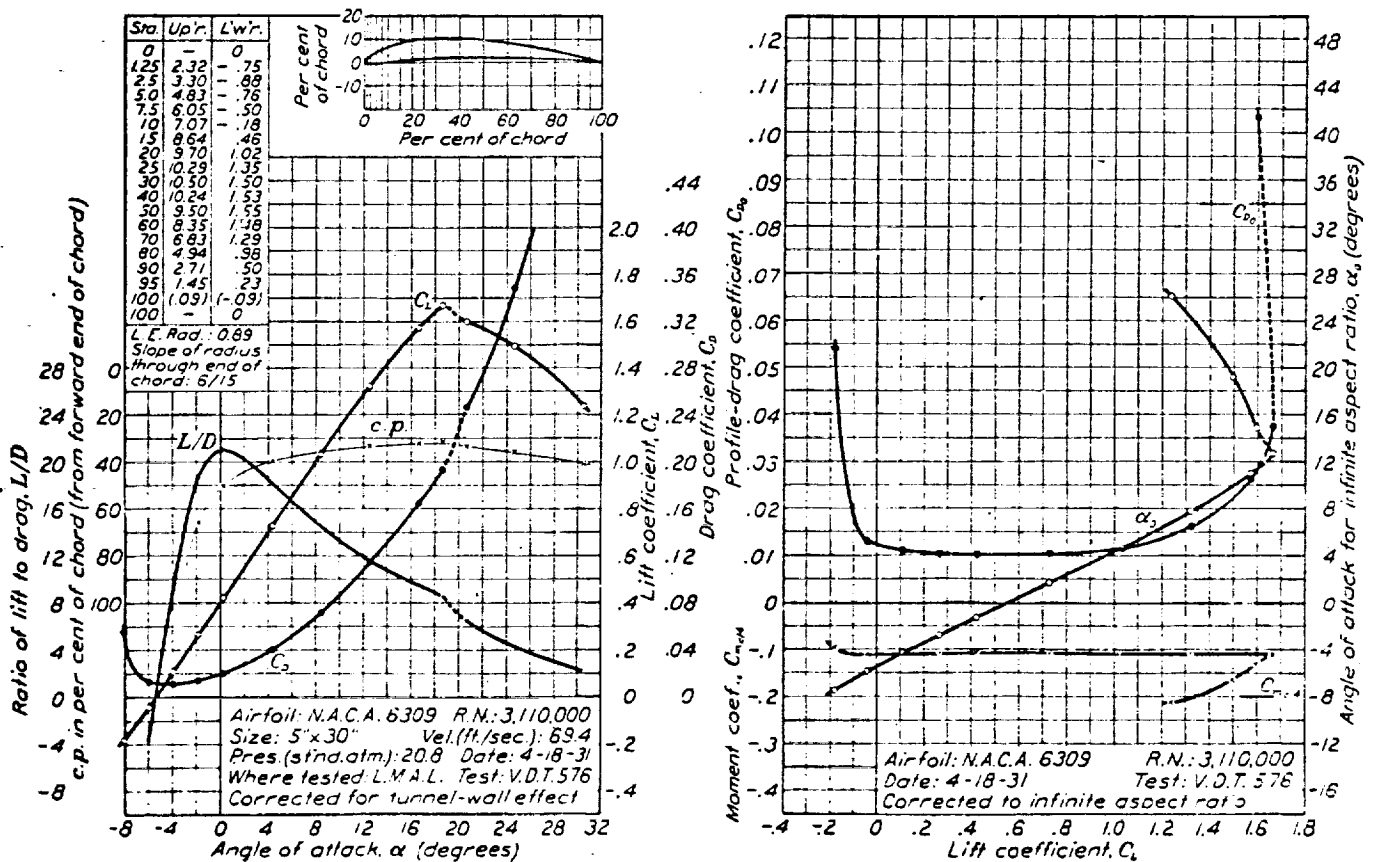
FIGURE 53.—N.A.C.A. 6309 airfoil.
