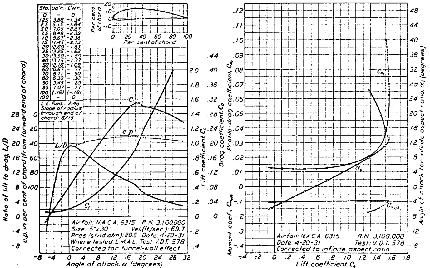
FIGURE 55.—N.A.C.A. 6315 airfoil.
