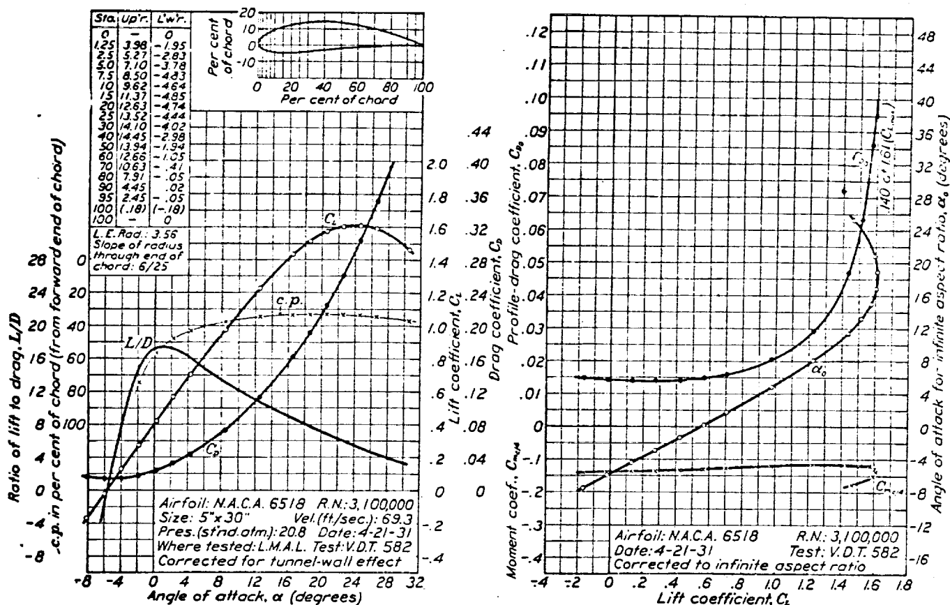
FIGURE 68.—N.A.C.A. 6518 airfoil.
