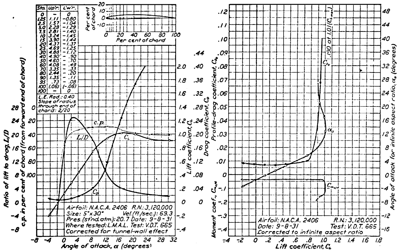
FIGURE 16.—N.A.C.A. 2406 airfoil.
