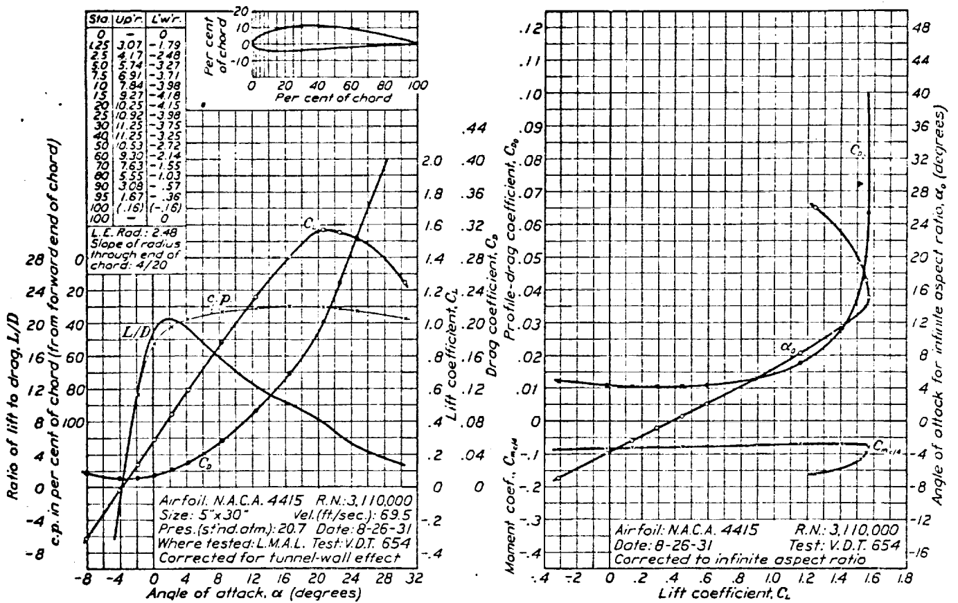
FIGURE 40.—N.A.C.A. 4415 airfoil.
