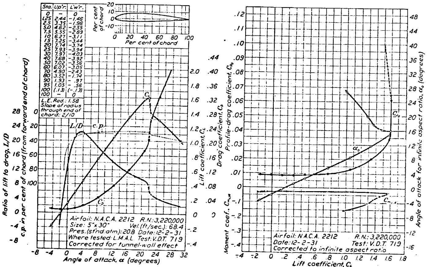
FIGURE 11.—N.A.C.A. 2212 airfoil.
