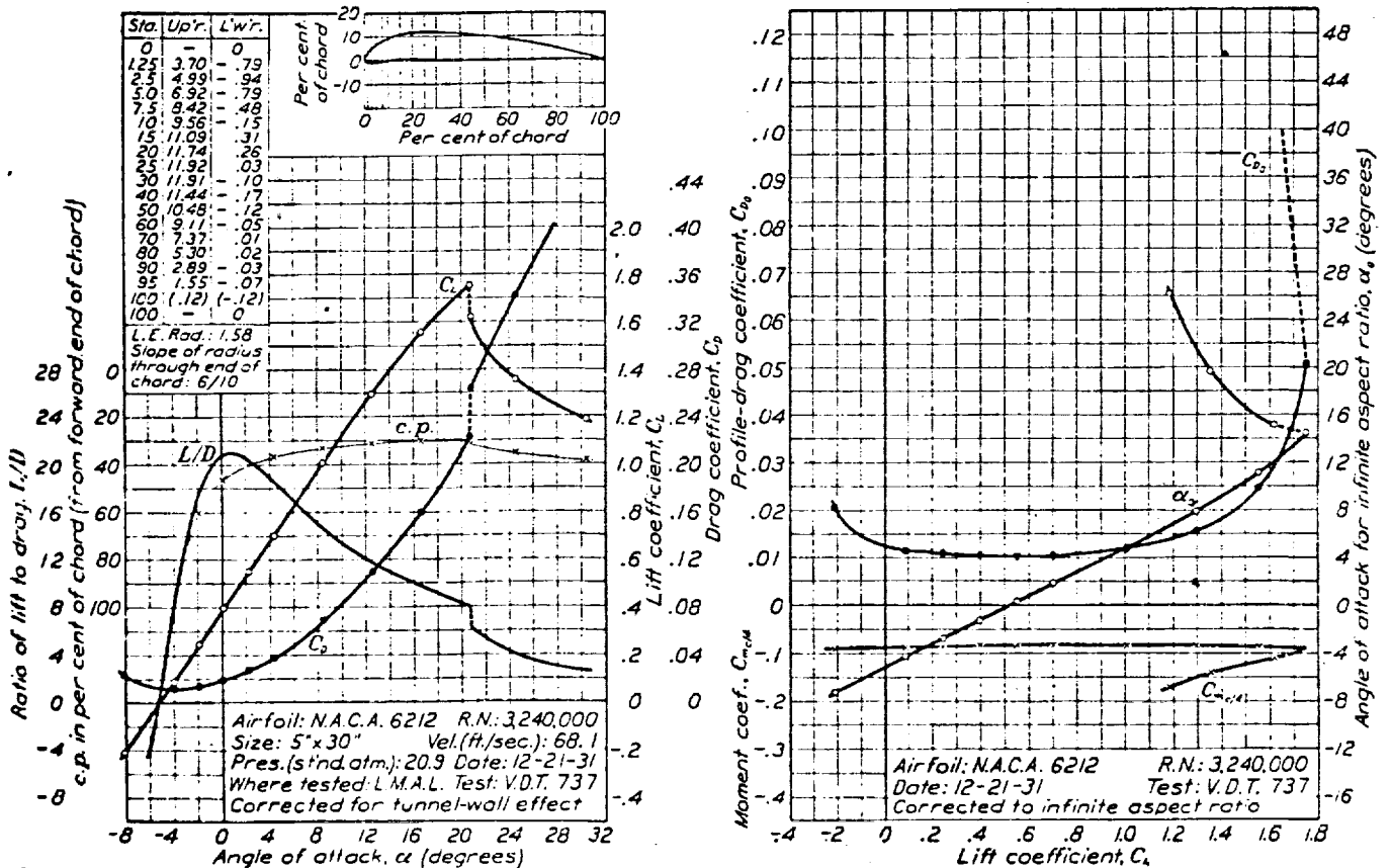
FIGURE 51.—N.A.C.A. 6212 airfoil.
