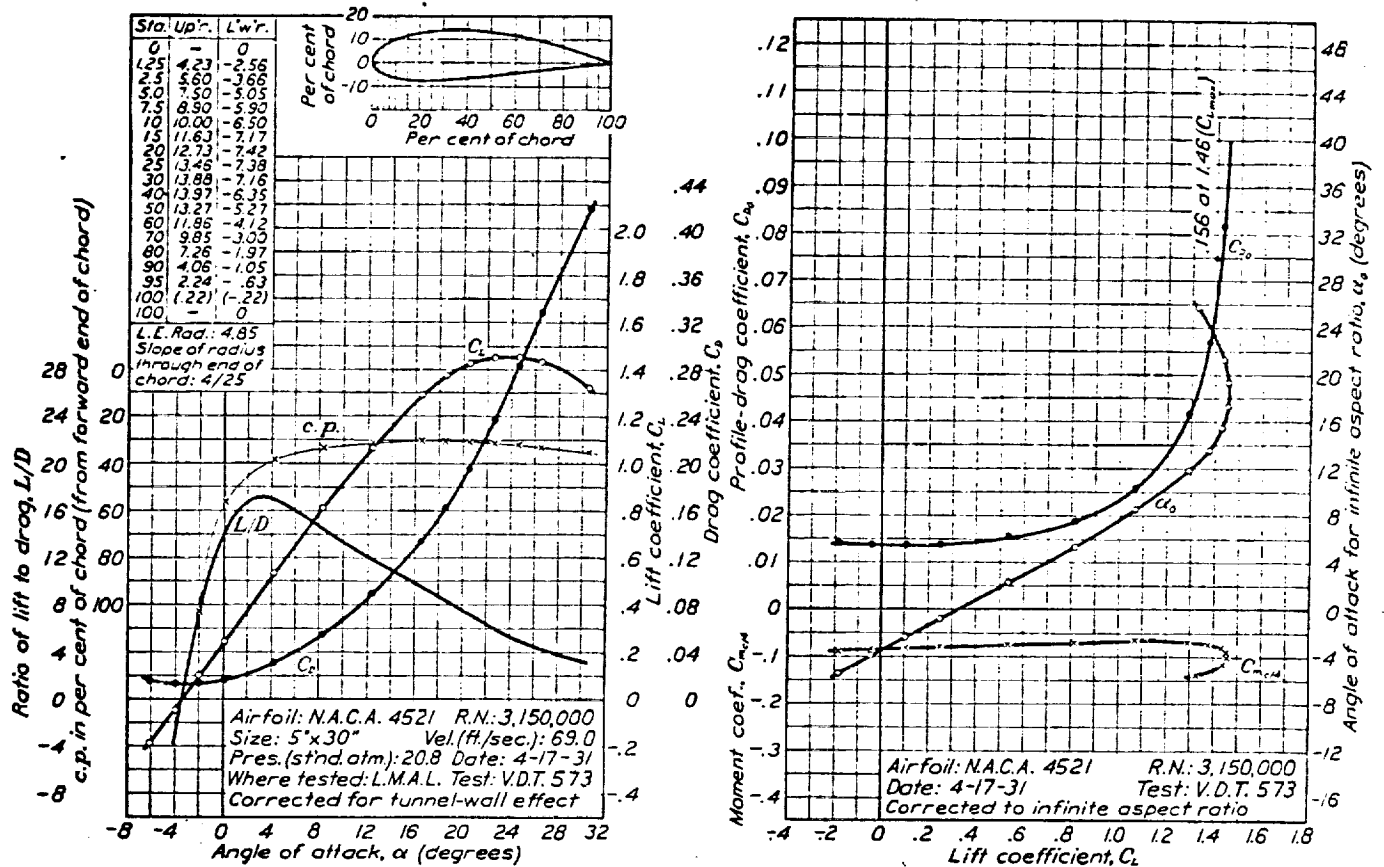
FIGURE 48.—N.A.C.A. 4521 airfoil.
