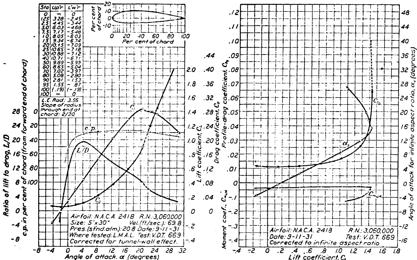
FIGURE 20.—N.A.C.A. 2418 airfoil.
