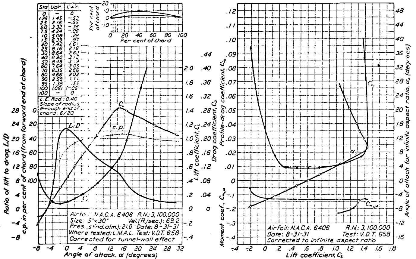
FIGURE 58.—N.A.C.A. 6406 airfoil.
