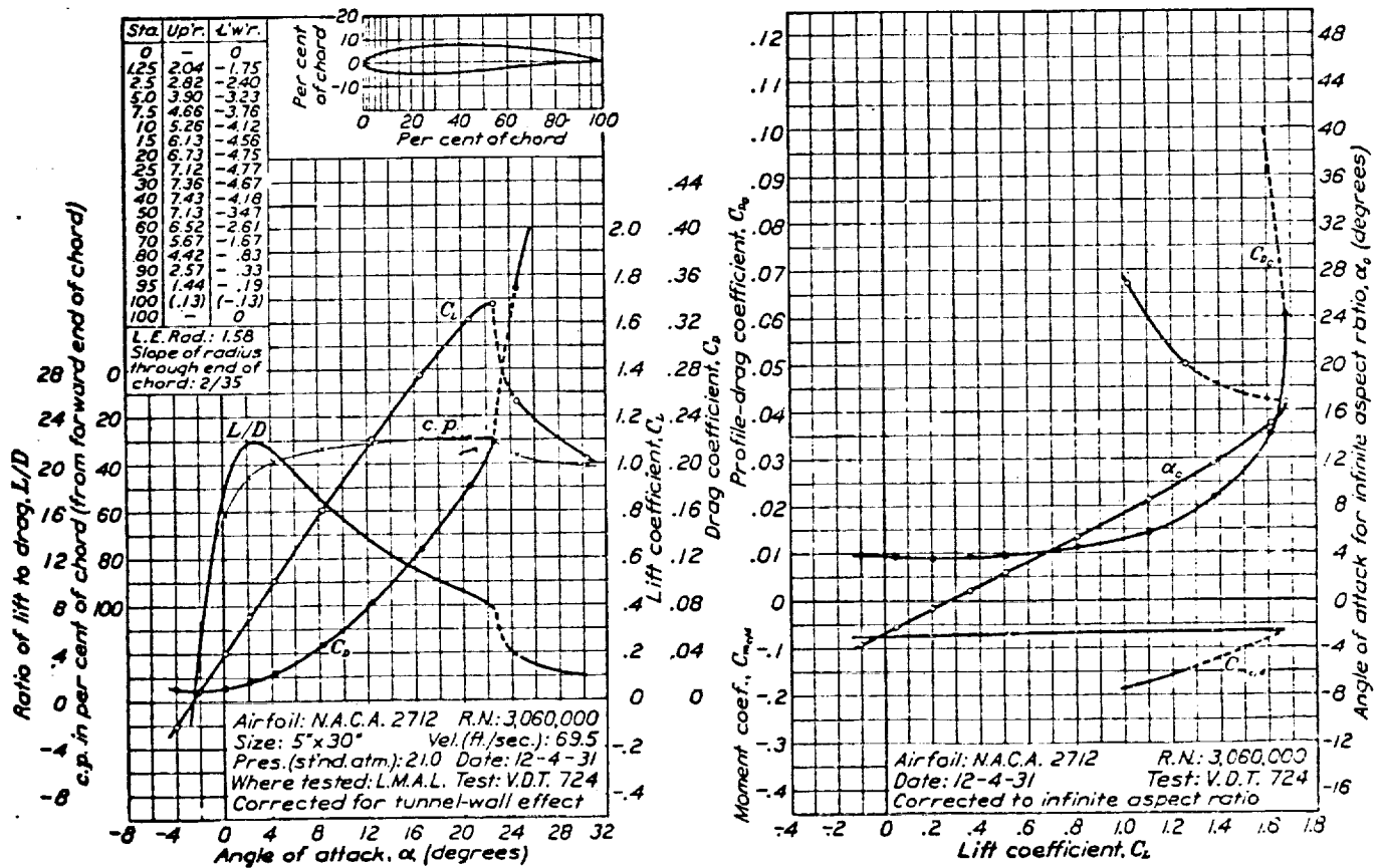
FIGURE 2B.—N.A.C.A. 2712 airfoil.
