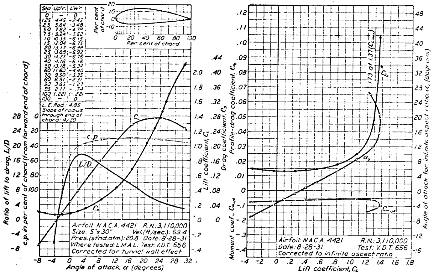
FIGURE 42.—N.A.C.A. 4421 airfoil.
