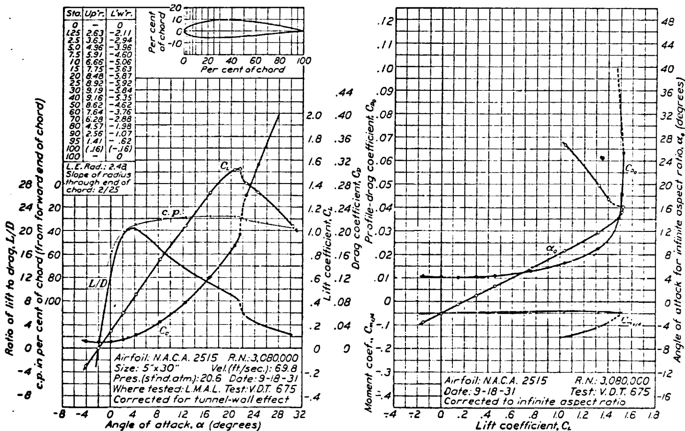
FIGURE 25.—N.A.C.A. 2515 airfoil.
