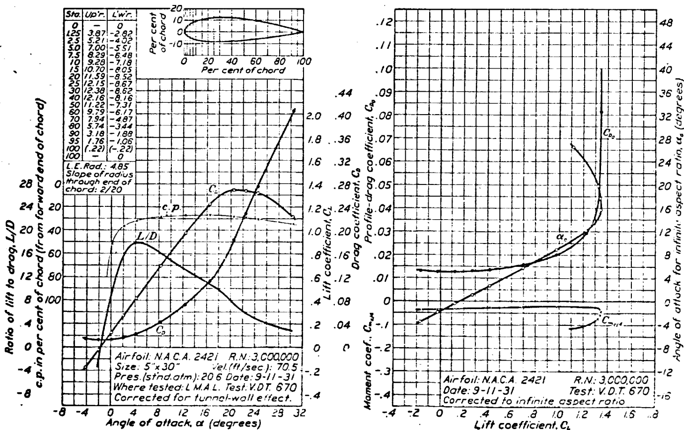
FIGURE 21.—N.A.C.A. 2421 airfoil.
