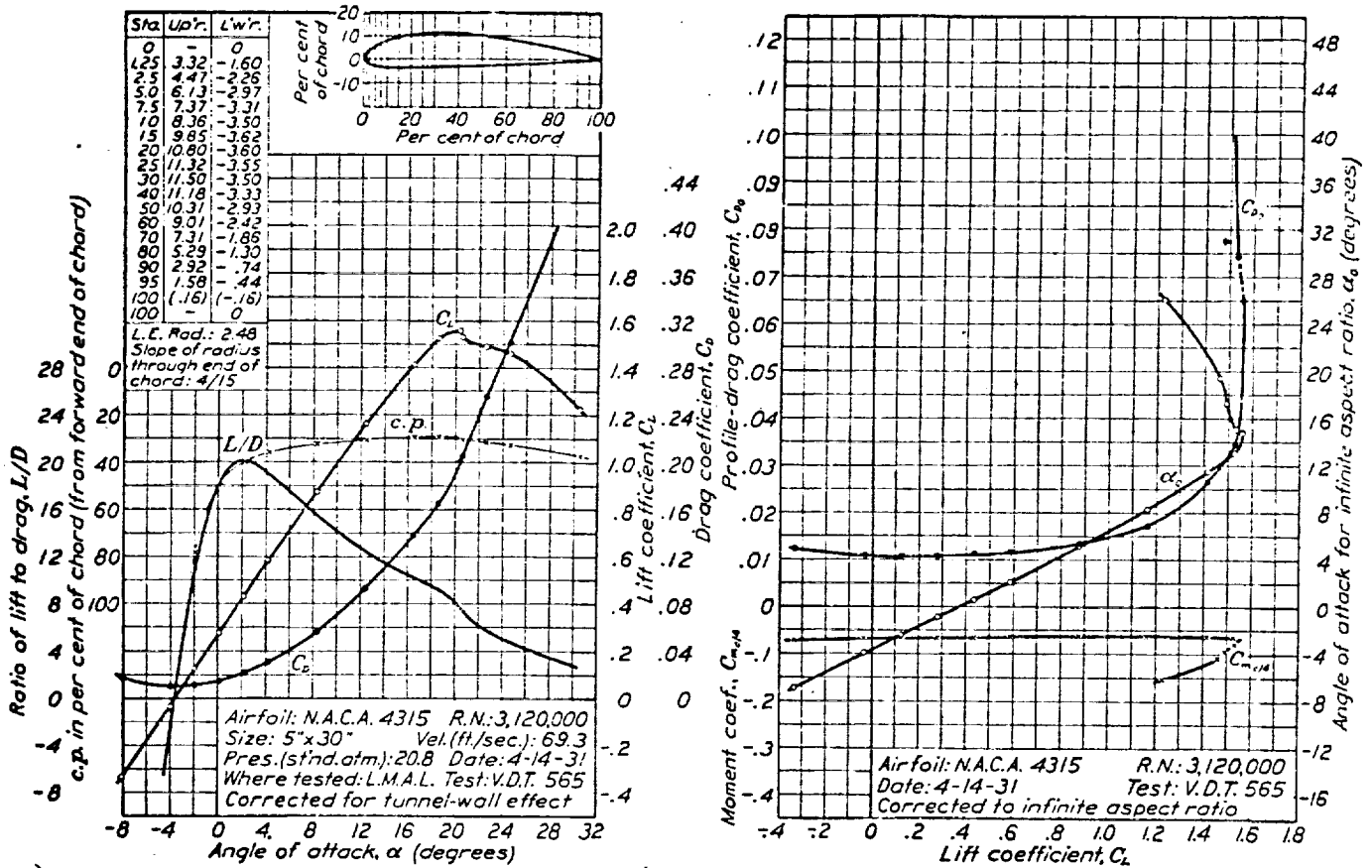
FIGURE 34.—N.A.C.A. 4315 airfoil.
