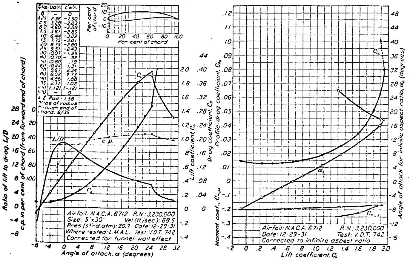
FIGURE 71.—N.A.C.A. 6712 airfoil.
