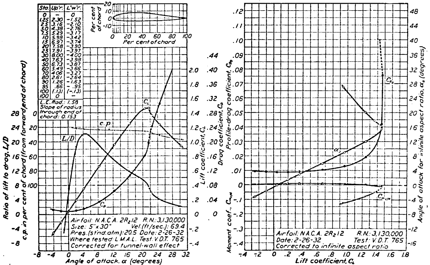
FIGURE 79.—N.A.C.A. 2R 2 airfoil.
