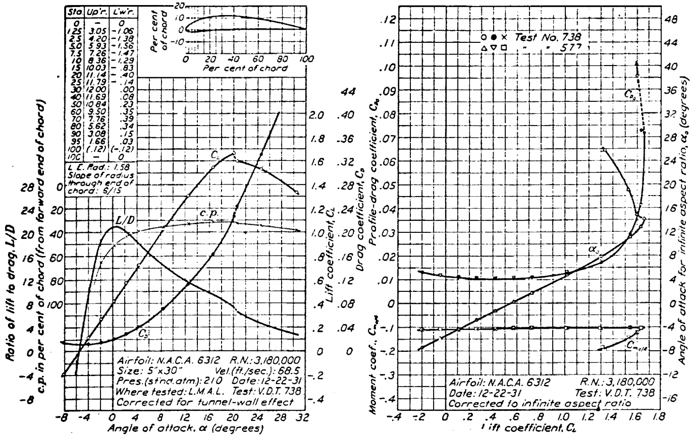
FIGURE 54.—N.A.C.A. 6312 airfoil.
