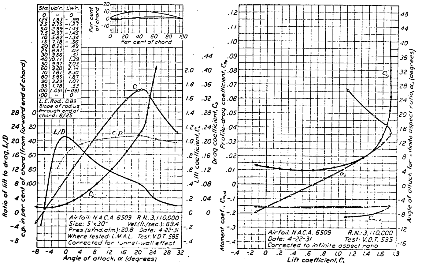
FIGURE 65.—N.A.C.A. 6509 airfoil.
