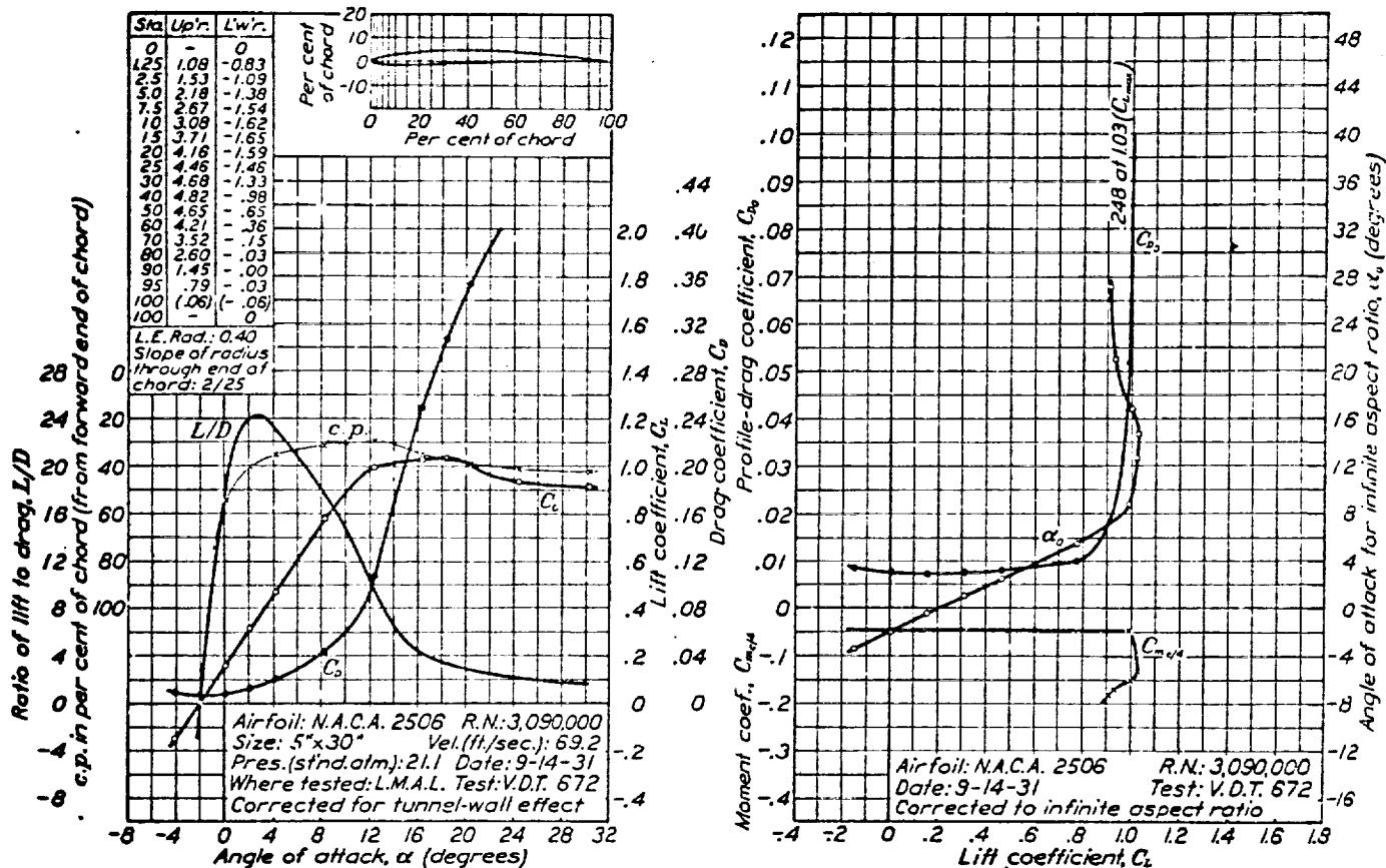
FIGURE 22.—N.A.C.A. 2506 airfoil.
