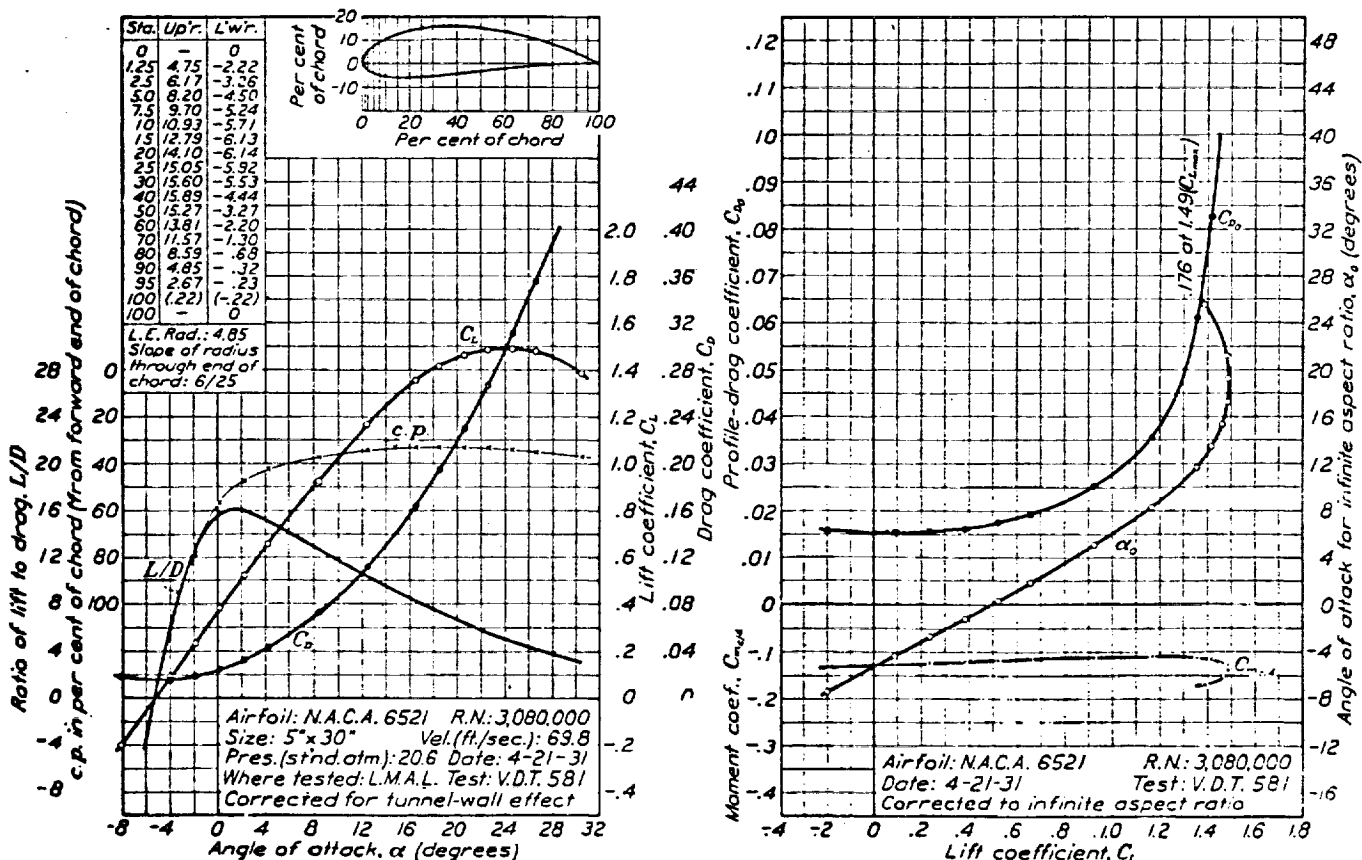
FIGURE 69.—N.A.C.A. 6521 airfoil.
