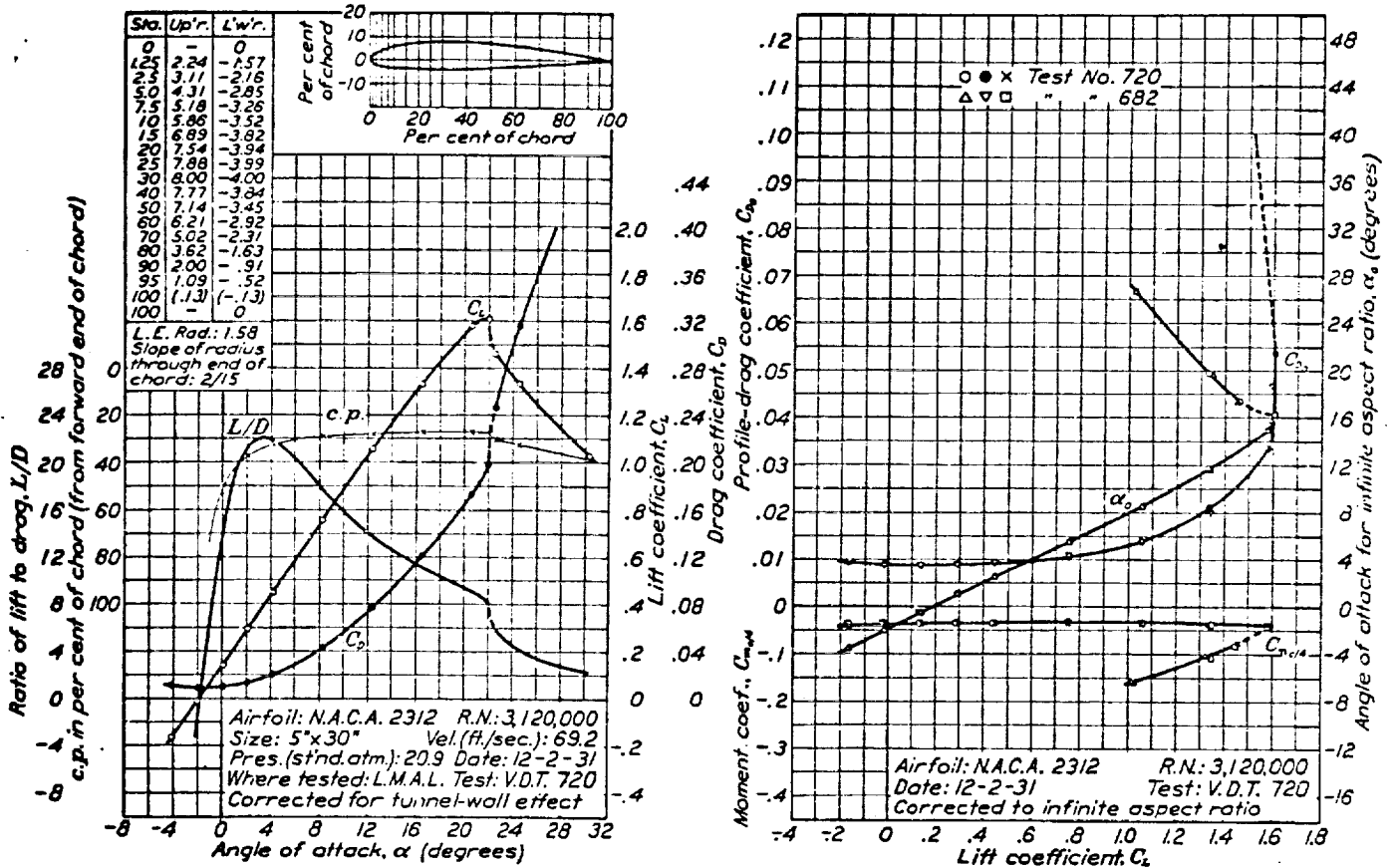
FIGURE 14.—N.A.C.A. 2312 airfoil.
