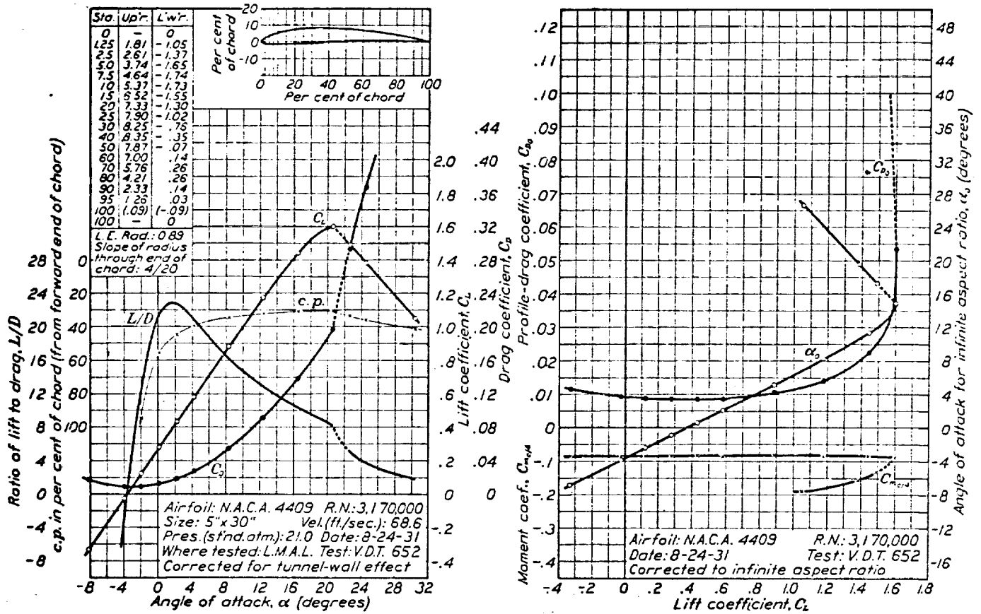
FIGURE 38.—N.A.C.A. 4409 airfoil.
