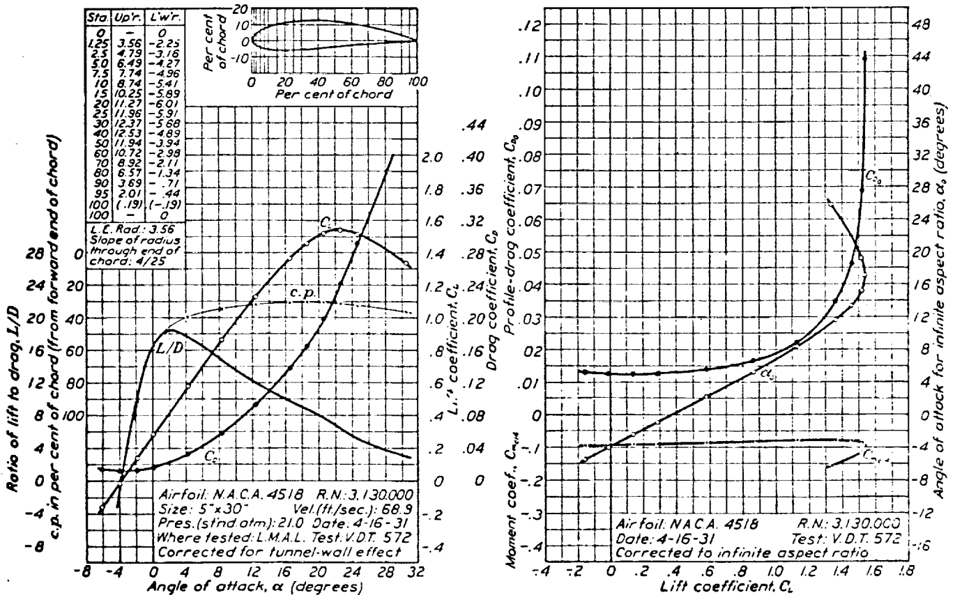
FIGURE 47.—N.A.C.A. 4518 airfoil.
