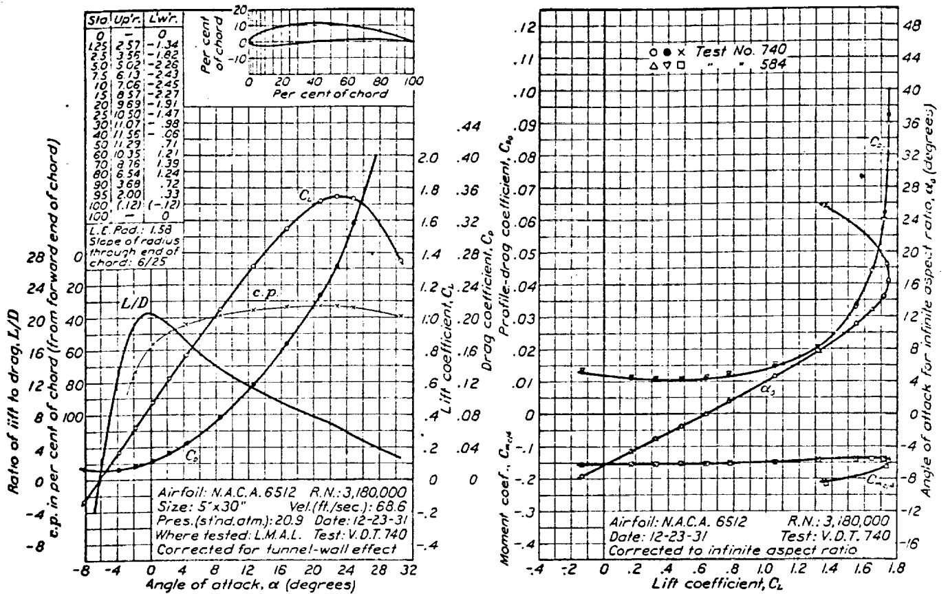
FIGURE 66.—N.A.C.A. 6512 airfoil.
