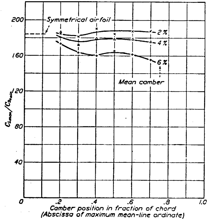
FIGURE 96.—Variation of C_{L_{max}}/C_{D_{0.05}} with camber. Results are for 12 percent thick airfoils.
