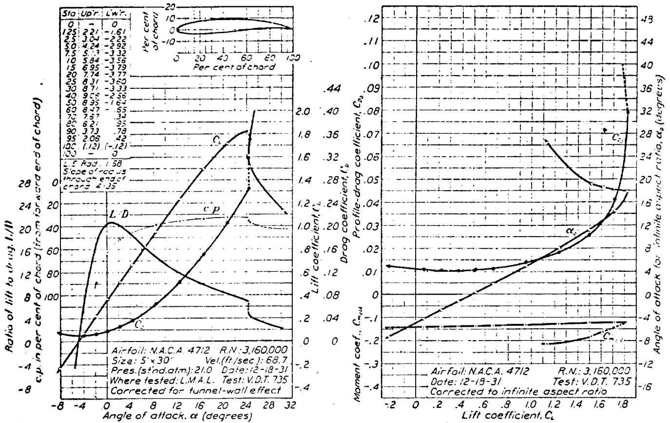
FIGURE 50.—N.A.C.A. 4712 airfoil.
