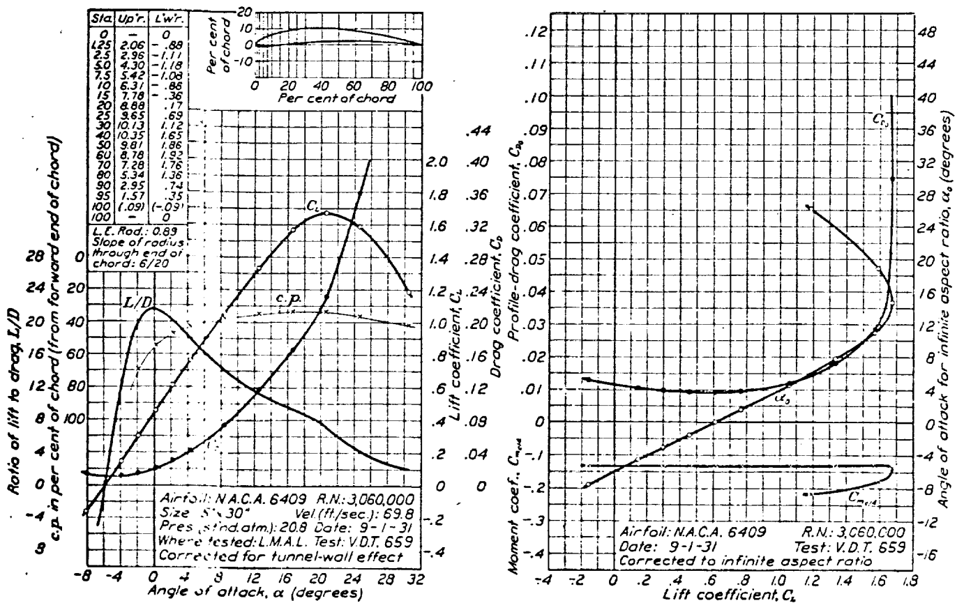
FIGURE 59.—N.A.C.A. 6409 airfoil.
