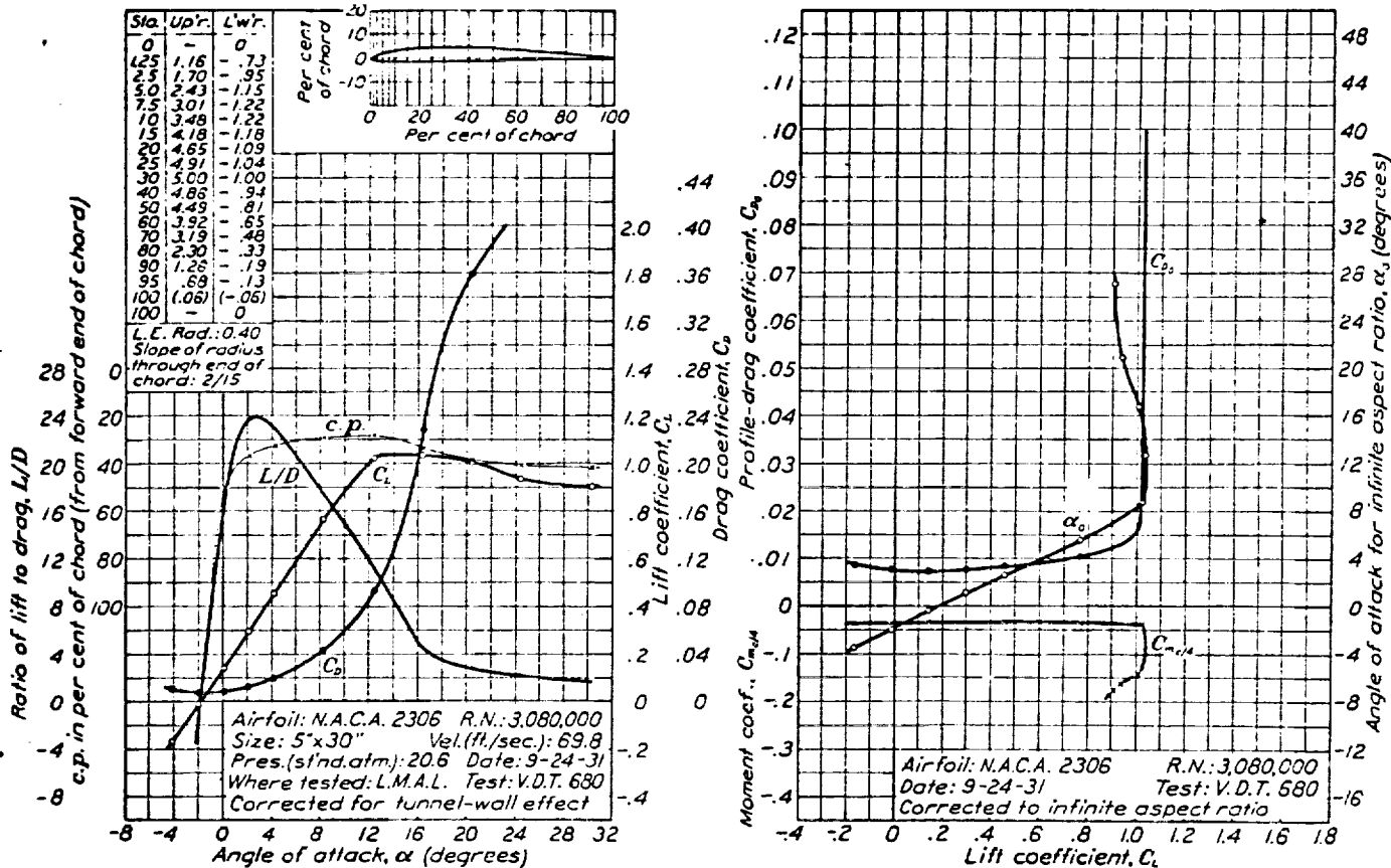
FIGURE 12.—N.A.C.A. 2306 airfoil.
