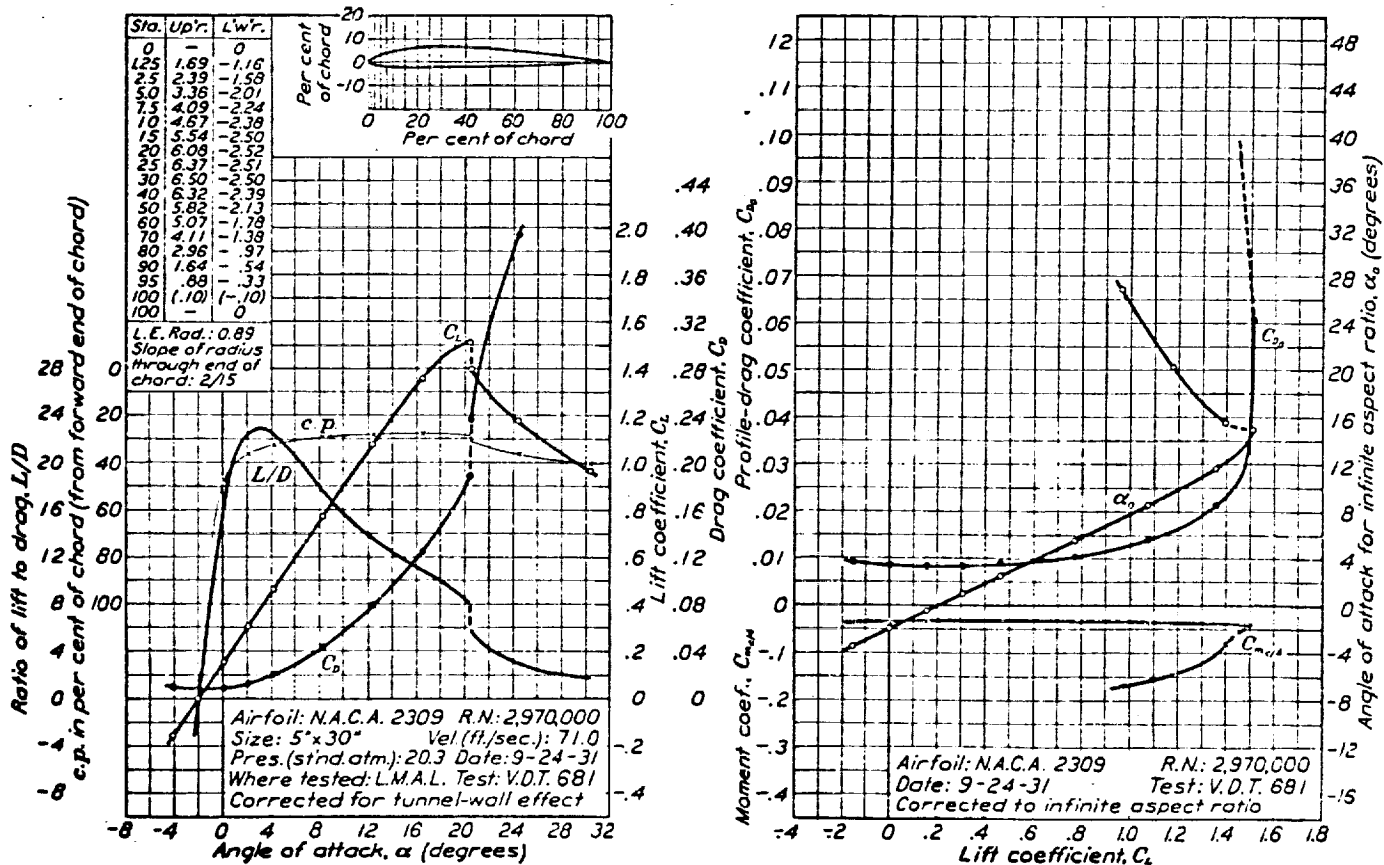
FIGURE 13.—N.A.C.A. 2309 airfoil.
