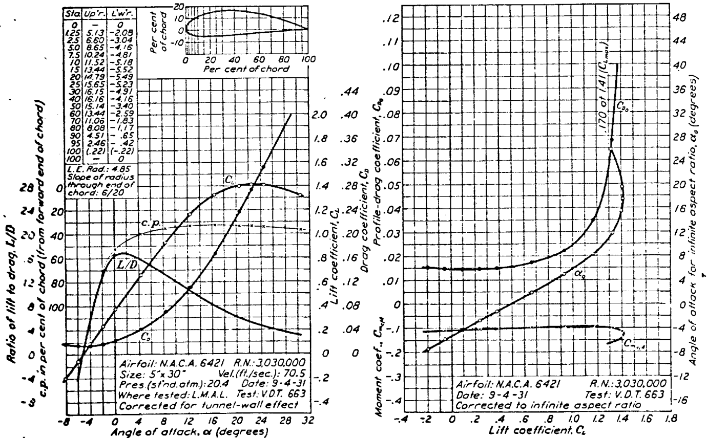
FIGURE 63.—N.A.C.A. 6421 airfoil.
