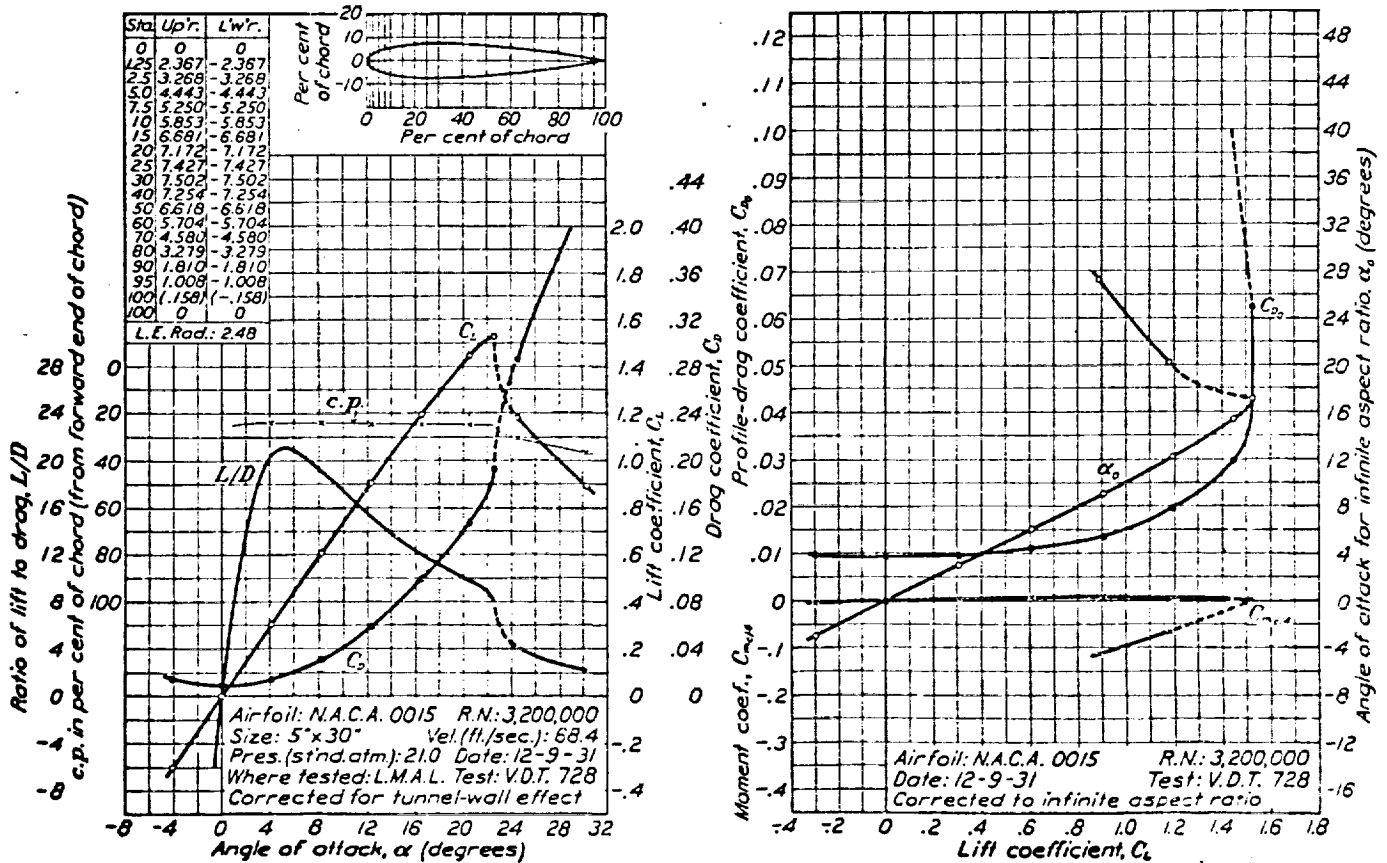
FIGURE 7.—N.A.C.A. 0015 airfoil.
