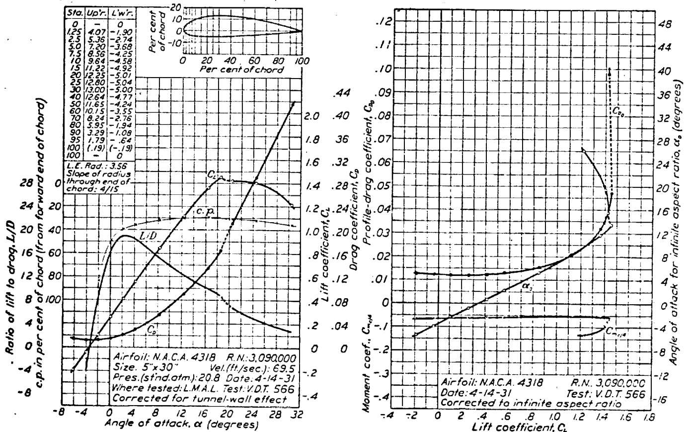
FIGURE 35.—N.A.C.A. 4318 airfoil.
