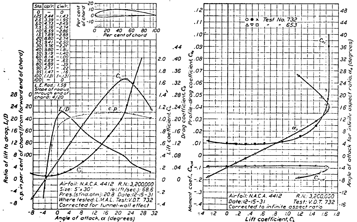
FIGURE 39.—N.A.C.A. 4412 airfoil.
