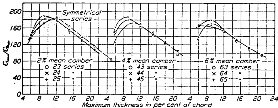
FIGURE 95.—Variation of C_{L_{max}}/C_{D_{0.05}} with thickness.
