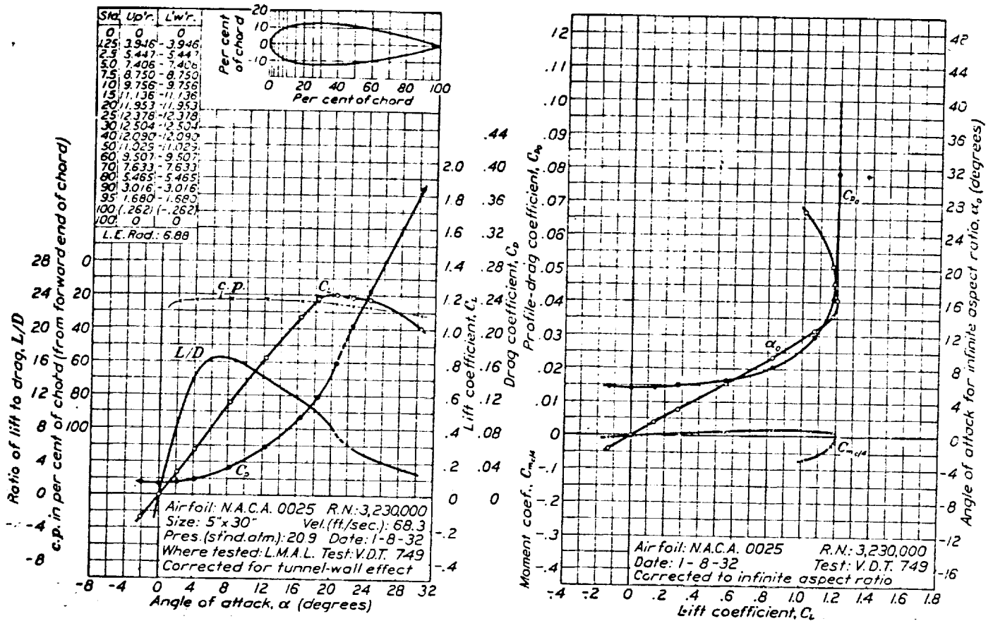
FIGURE 10.—N.A.C.A. 0025 airfoil.
