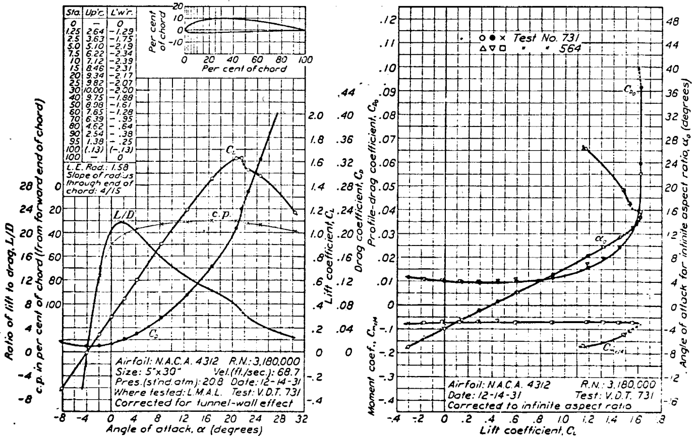
FIGURE 33.—N.A.C.A. 4312 airfoil.
