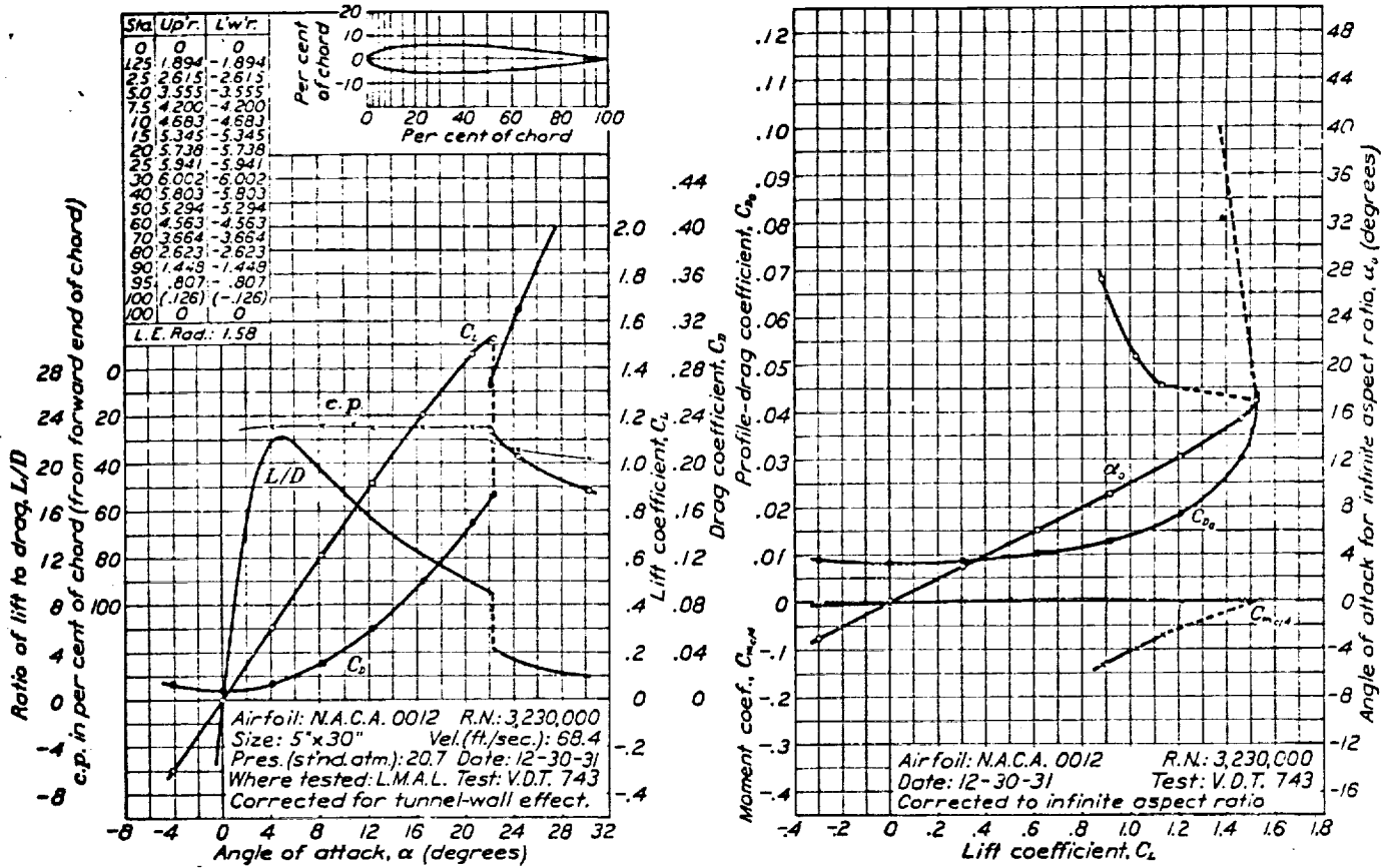
FIGURE 6.—N.A.C.A. 0012 airfoil.
