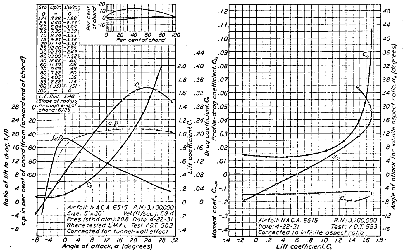
FIGURE 67.—N.A.C.A. 6515 airfoil.
