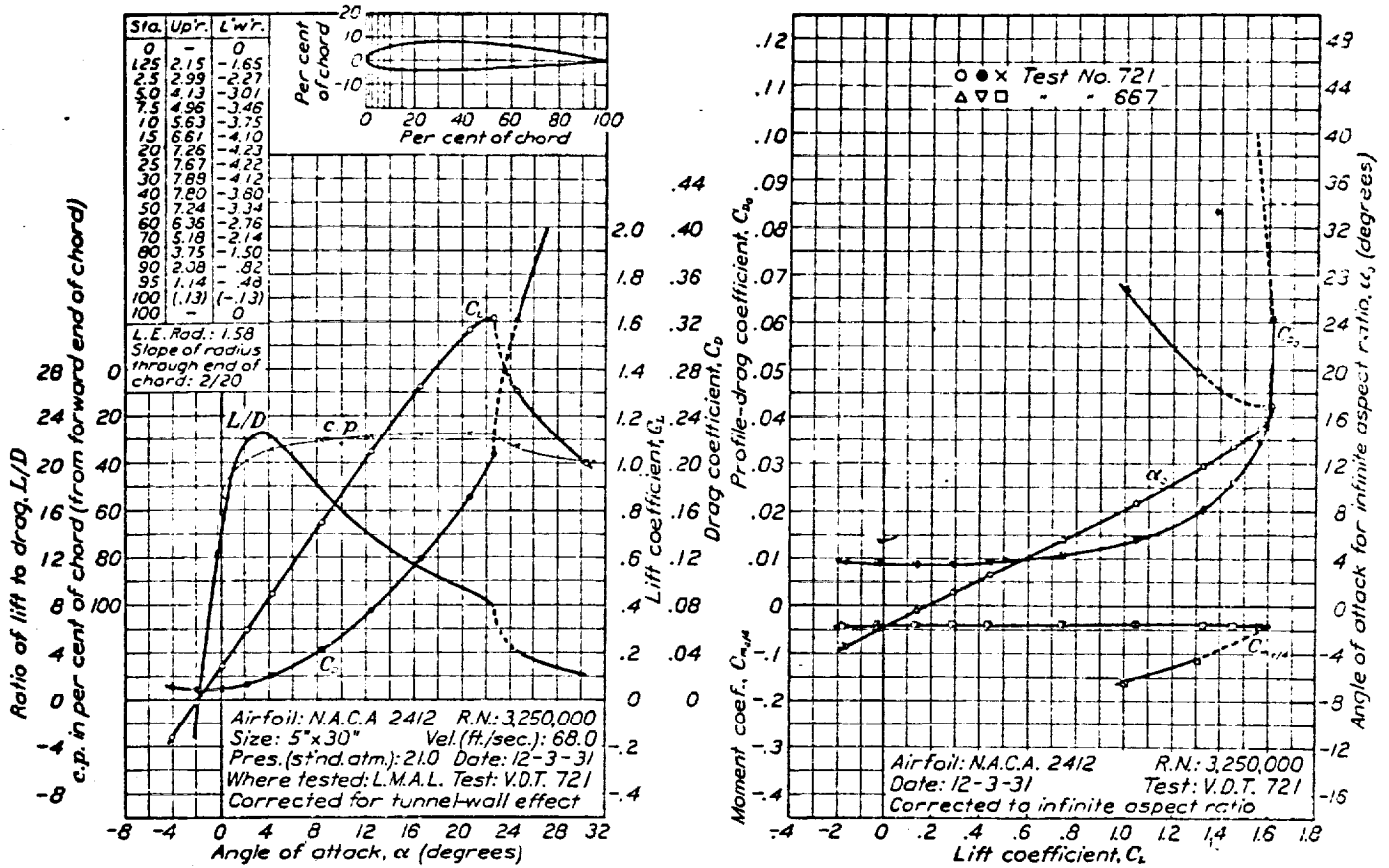
FIGURE 18.—N.A.C.A. 2412 airfoil.
