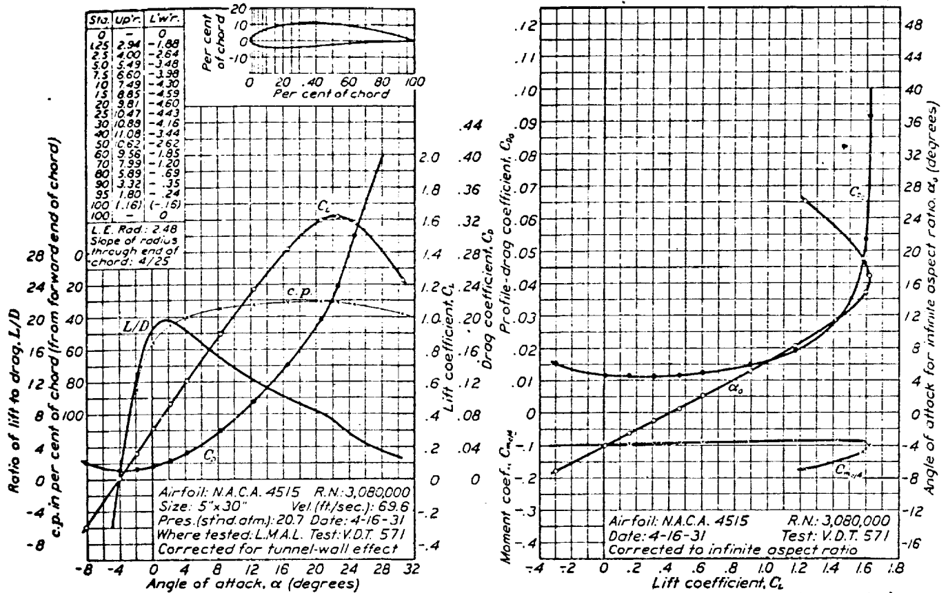
FIGURE 46.—N.A.C.A. 4515 airfoil.
