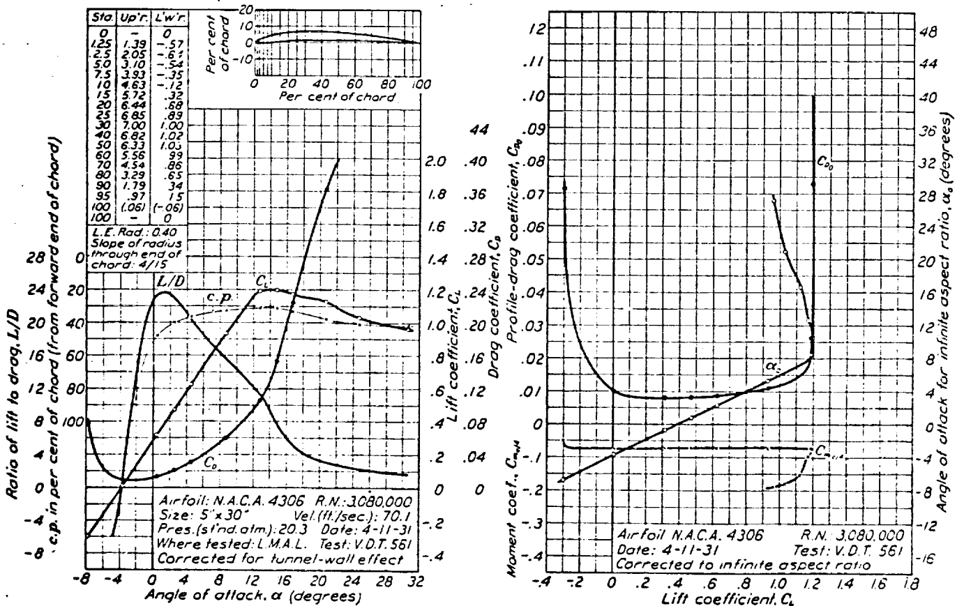
FIGURE 31.—N.A.C.A. 4306 airfoil.
