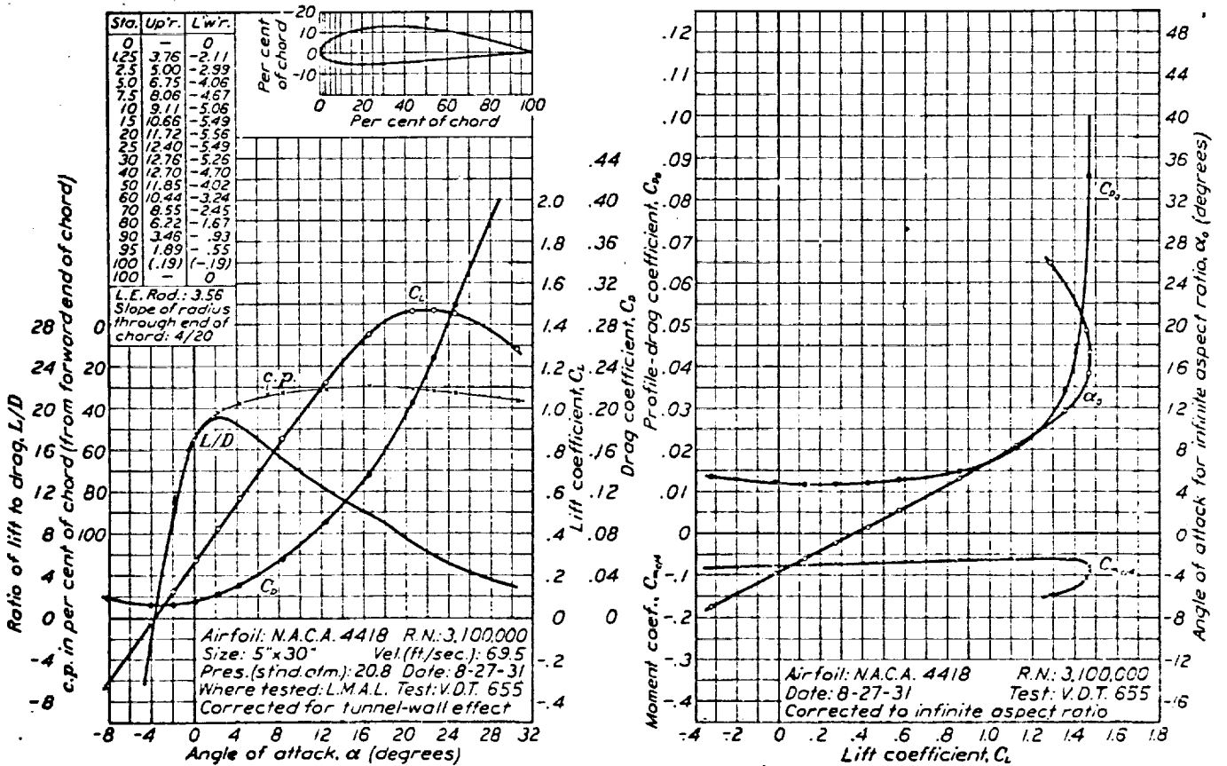
FIGURE 41.—N.A.C.A. 4418 airfoil.
