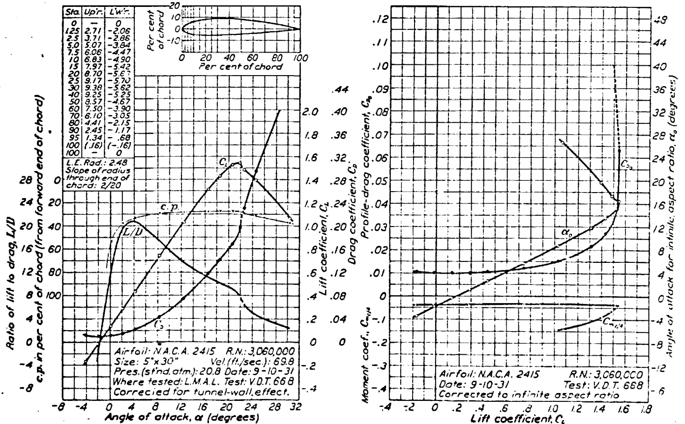
FIGURE 19.—N.A.C.A. 2415 airfoil.
