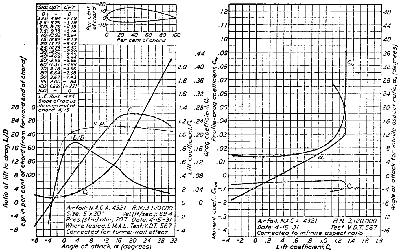
FIGURE 36.—N.A.C.A. 4321 airfoil.
