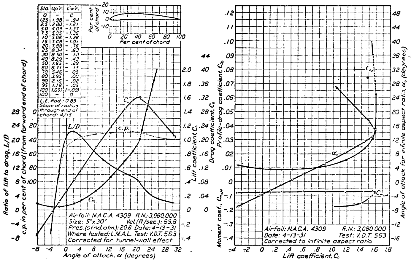
FIGURE 32.—N.A.C.A. 4309 airfoil.
