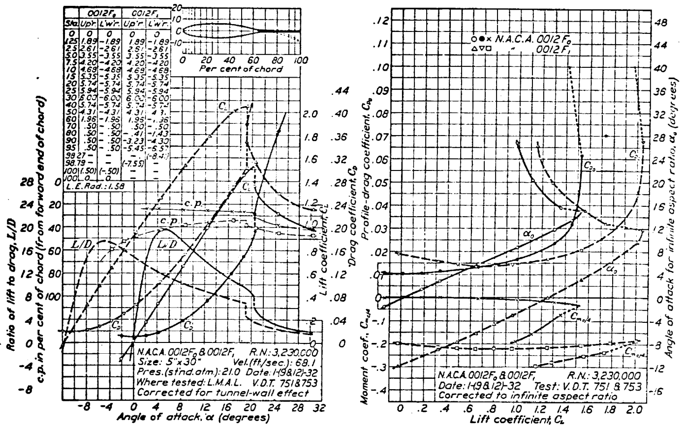
FIGURE 80.—N.A.C.A. 0012F 0 and 0012F 1 airfoils.
