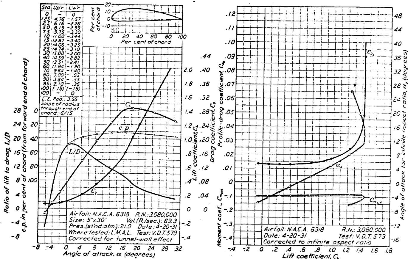
FIGURE 56.—N.A.C.A. 6318 airfoil.
