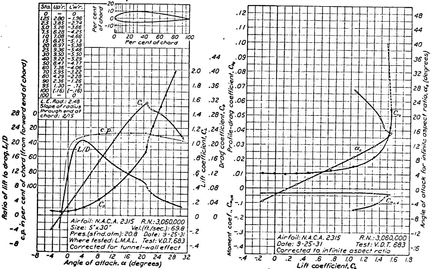
FIGURE 15.—N.A.C.A. 2315 airfoil.
