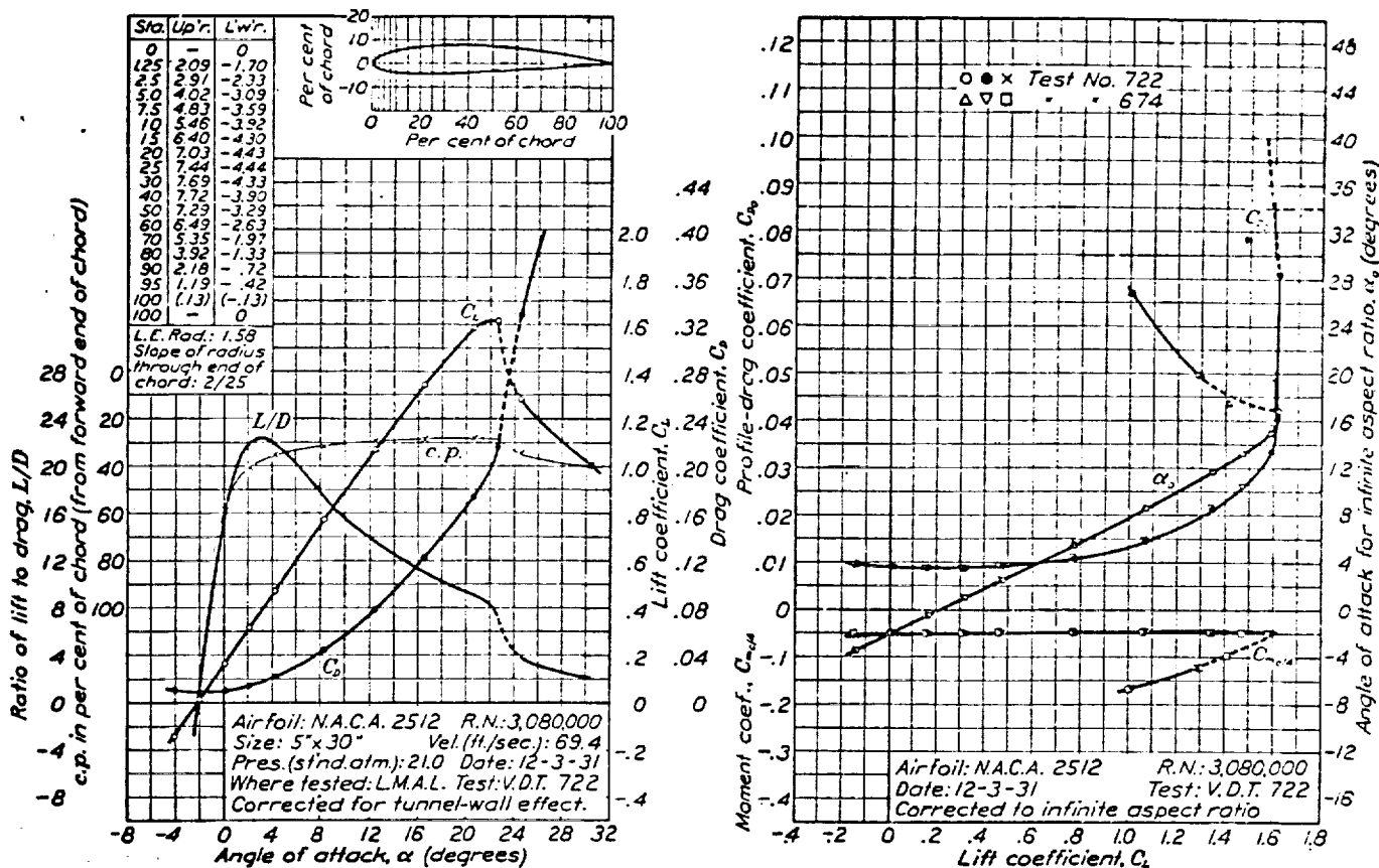
FIGURE 24.—N.A.C.A. 2512 airfoil.
