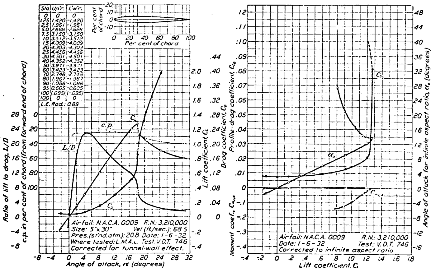
FIGURE 5.—N.A.C.A. 0009 airfoil.
