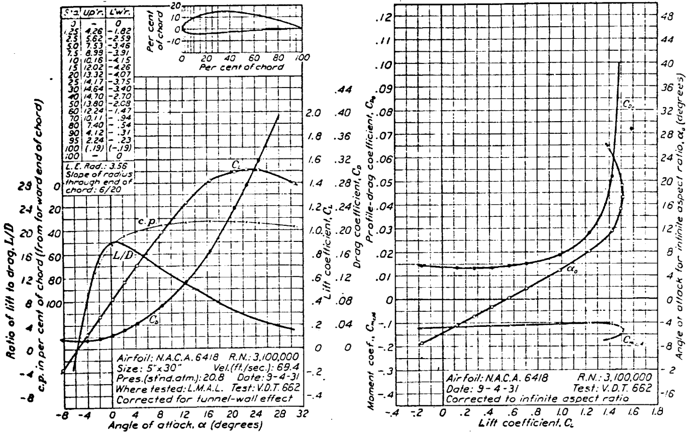
FIGURE 62.—N.A.C.A. 6418 airfoil.
