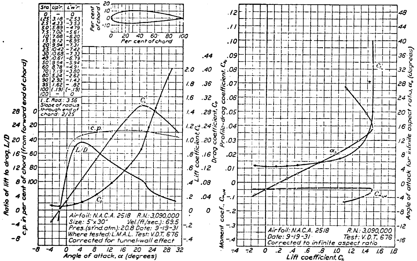
FIGURE 26.—N.A.C.A. 2518 airfoil.
