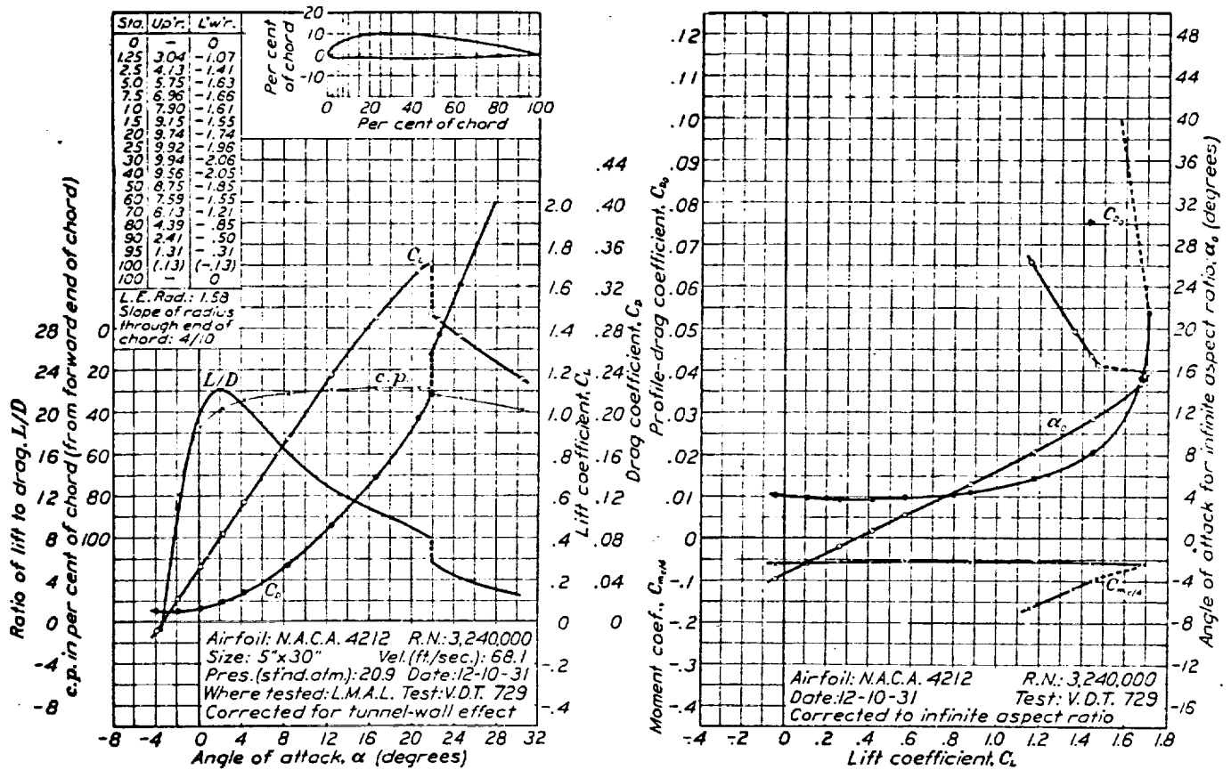
FIGURE 30.—N.A.C.A. 4212 airfoil.
