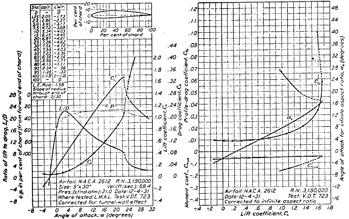
FIGURE 2A.—N.A.C.A. 2612 airfoil.
